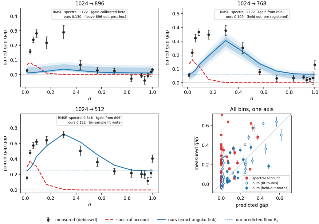
Figure 2: Both accounts on the same axes. Per route, one set of measured debiased gap curves (Eq. 1, black) carries both predictions of §3: the spectral account (red dashed; transported through the residual→gradient bridge at the measured anchor tolerance — the whole family scores alike, Appendix Fig. 6) and ours under the exact angular link (blue, Eq. 18; three-form comparison in Appendix Fig. 4), with each route’s predicted floor (blue dashed — dashed-to-solid is the data term) and a 68%/95% full-pipeline bootstrap band ( B=1000 ; Appendix B). Neither account is fit to the route it is drawn on except as labelled in-panel: ours predicts 1024→768 from governors alone with zero per-route freedom (pre-registered held-out) and 1024→896 under the post-hoc leave-896-out re-derivation, while the spectral account’s single gain is calibrated on 1024→896 and frozen. The 768 mid- \sigma dip and the 896 low- \sigma plateau sit outside the 95% band — the two edges of the reduction’s domain (Appendix C). Bottom right: predicted vs measured over every bin, with ours also on the two 1280-tier routes the spectral bridge does not cover.
