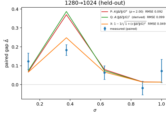
Figure 4: The second held-out route, 1280→1024, under all three functional forms for the data term of Appendix C (fitted power, derived quadratic, exact angular link; legend G := \|\bar{g}_{\text{src}}(\sigma)\| ), predicted from governors fitted on other routes. This is the one route where the forms visibly separate: the derived quadratic systematically overshoots the mid- \sigma peak; the exact angular link’s saturation removes the overshoot (RMSE 0.049 vs \approx 0.095 ), which is why the exact link headlines in Fig. 2.
