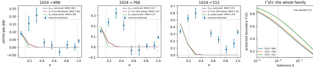
Figure 6: The whole tolerance family against the measurement — the detail behind the single red curve of Fig. 2. Left three panels: the measured debiased gap curves against the spectral account transported through our bridge (the diagonal model's destroyed-band mean-residual mismatch on the measured spectrum, through the measured \|\tilde{g}_{src}(\sigma)\| with a single gain calibrated on the one safe route and no floor — the family expresses none), gated at t^*(\delta) (dashed verticals) for the equal-power slice, SPD's default \delta = 0.01 , and the measured anchor \delta_{reenc} . The transported curve dies by \sigma \approx 0.35 on every route, so the two larger gates (0.61–0.72 and 0.98–0.99) act on an already-zero curve and coincide exactly; the equal-power gate (0.14–0.20) is the only one that truncates live curve, and it moves RMSE by at most 0.008. All three therefore land within 0.01 of each other: \delta is inert at the curve level. Right: the boundary family t^*(\delta) ; maximum route spread 0.125 in \sigma over \delta \in [10^{-3}, 0.5] .
