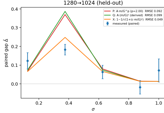
Figure 4: The second held-out route, 1280→1024, under all three functional forms for the data term of §4.6 (fitted power, derived quadratic, exact angular link), predicted from governors fitted on other routes. This is the one route where the forms visibly separate: the derived quadratic systematically overshoots the mid- \sigma peak; the exact angular link’s saturation removes the overshoot (RMSE 0.049 vs \approx 0.095 ), which is why the exact link headlines in Fig. 2.
