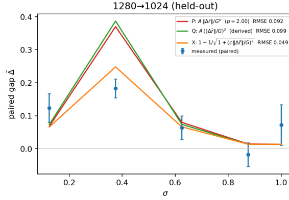
Figure 3: The second held-out route, 1280→1024, under all three functional forms for the data term of §4.4 (fitted power, derived quadratic, exact angular link; legend G := \|\bar{g}_{\text{src}}(\sigma)\| ), predicted from governors fitted on other routes. This is the one route where the forms visibly separate: the derived quadratic systematically overshoots the mid- \sigma peak; the exact angular link’s saturation removes the overshoot (RMSE 0.049 vs \approx 0.095 ), which is why the exact link headlines in Fig. 1.
