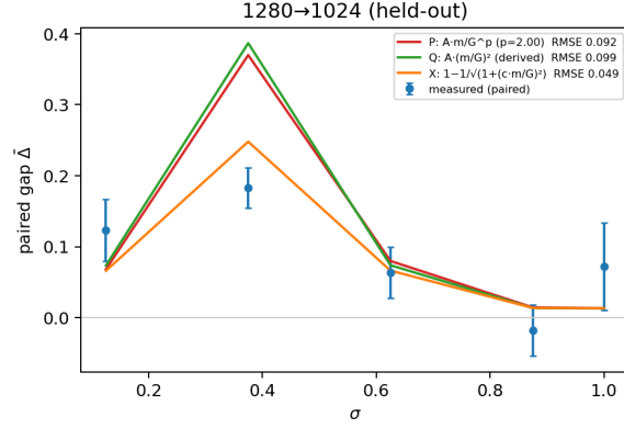
Figure 4: The second held-out route, 1280→1024, under all three functional forms for the data term of §4.5 (fitted power, derived quadratic, exact angular link), predicted from governors fitted on other routes. This is the one route where the forms visibly separate: the derived quadratic systematically overshoots the mid- \sigma peak; the exact angular link’s saturation removes the overshoot (RMSE 0.049 vs \approx 0.095 ), which is why the exact link headlines in Fig. 2.
