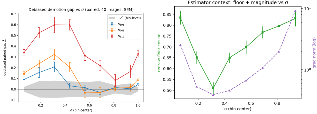
Figure 3: The measurement in detail. (a) Debiased demotion gap per \sigma -bin, paired against the re-encoding control (1024-tier natives, N=40 ; per-bin values and SEMs in Appendix Table 7; gray band: bin-level \pm\epsilon^* , Eq. 2; open markers: the \sigma=1 endpoint bin): safety is a per-route boundary — the 896 route enters the band at \sigma \approx 0.5 , 768 has no certifiable window, and 512 does not enter at any noise level — against the spectral family’s prediction of \sigma \approx 0.14\text{--}0.20 . (b) The estimator context those curves are read through: the redraw-floor cosine and the U-shaped gradient norm \|\tilde{g}_{\text{src}}(\sigma)\| .
