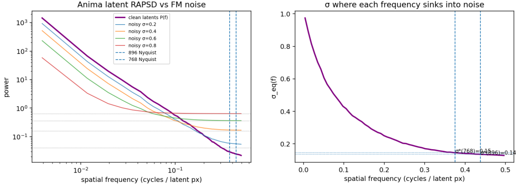
(a) Latent RAPSD against the flow-matching noise floor at four noise levels; dashed lines mark the demoted grids' Nyquist cuts.
