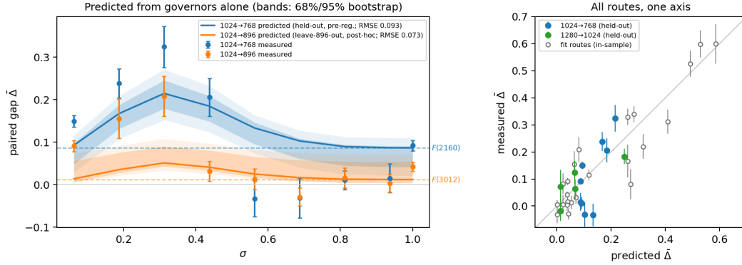
Figure 2: Our account against the same measurement , under the headline exact angular link (Eq. 5; three-form comparison in Appendix Fig. 4). Left: 1024-tier predictions with zero per-route freedom — the pre-registered held-out route 1024→768, and 1024→896 under the post-hoc leave-896-out re-derivation (so labeled; governors from 512+1120 alone). Dashed: each route’s predicted floor F(n) , so dashed-to-solid is the data term. Bands: 68%/95% full-pipeline bootstrap ( B=1000 ; Appendix D). The 768 mid- \sigma dip sits outside the 95% band and is the reduction’s one structural failure (§4.5). Right: predicted vs measured across all five routes and bins; filled: held-out, open: fit routes.
