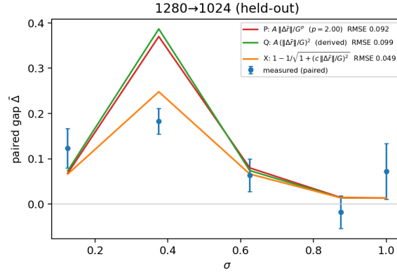
Figure 6: The second held-out route, 1280→1024, under all three functional forms for the data term of Appendix C (fitted power, derived quadratic, exact angular link; legend G := \|\bar{g}_{\text{src}}(\sigma)\| ), predicted from governors fitted on other routes. This is the one route where the forms visibly separate: the derived quadratic systematically overshoots the mid- \sigma peak; the exact angular link’s saturation removes the overshoot (RMSE 0.049 vs \approx 0.095 ), which is why the exact link is the form displayed in Fig. 2.
