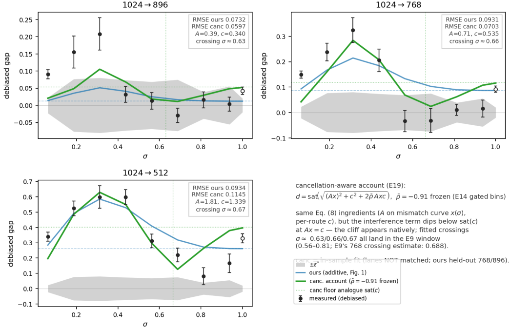
Figure 8: The cancellation-aware operational form (demonstration figure; in-sample). The exact link (Eq. 6) evaluated on both shares with the interference at the pooled constant \bar{\rho} = -0.91 , drawn over the measured curves: in-sample it reproduces the map’s shape including the 768 in-window dip below the route’s own floor, the structure the additive two-term form cannot express. This panel is a demonstration, not lane evidence; the lane-matched score (§4.4, identical protocol with only the link swapped) is: held-out 768 RMSE 0.078 vs. additive 0.099 with the dip placed at \sigma = 0.67 from held-out parameters alone; leave-one-out 896 lost at 0.086 vs. 0.077; 1280-tier guard broken on 1024 held-out (0.199 vs. 0.046). Reported at lane parity; not adopted — the additive lane keeps Fig. 2.
