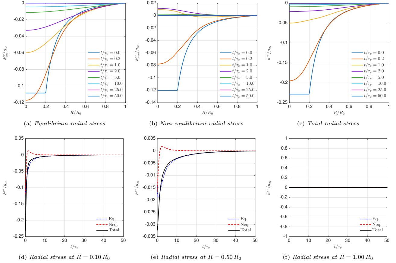
Figure 10: Radial stress. Top row: spatial profiles at selected times. Bottom row: time evolution at fixed material radii.
