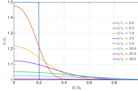
Figure 6: Temperature field \vartheta(R, t) at selected times.
