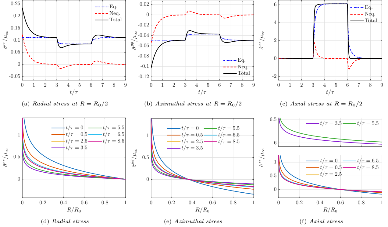
Figure 19: Force-controlled loading: stress evolution at fixed radius and stress radial profiles.
