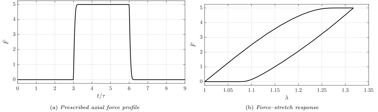
Figure 18: Force-controlled loading: global force response in time and in stretch space.
