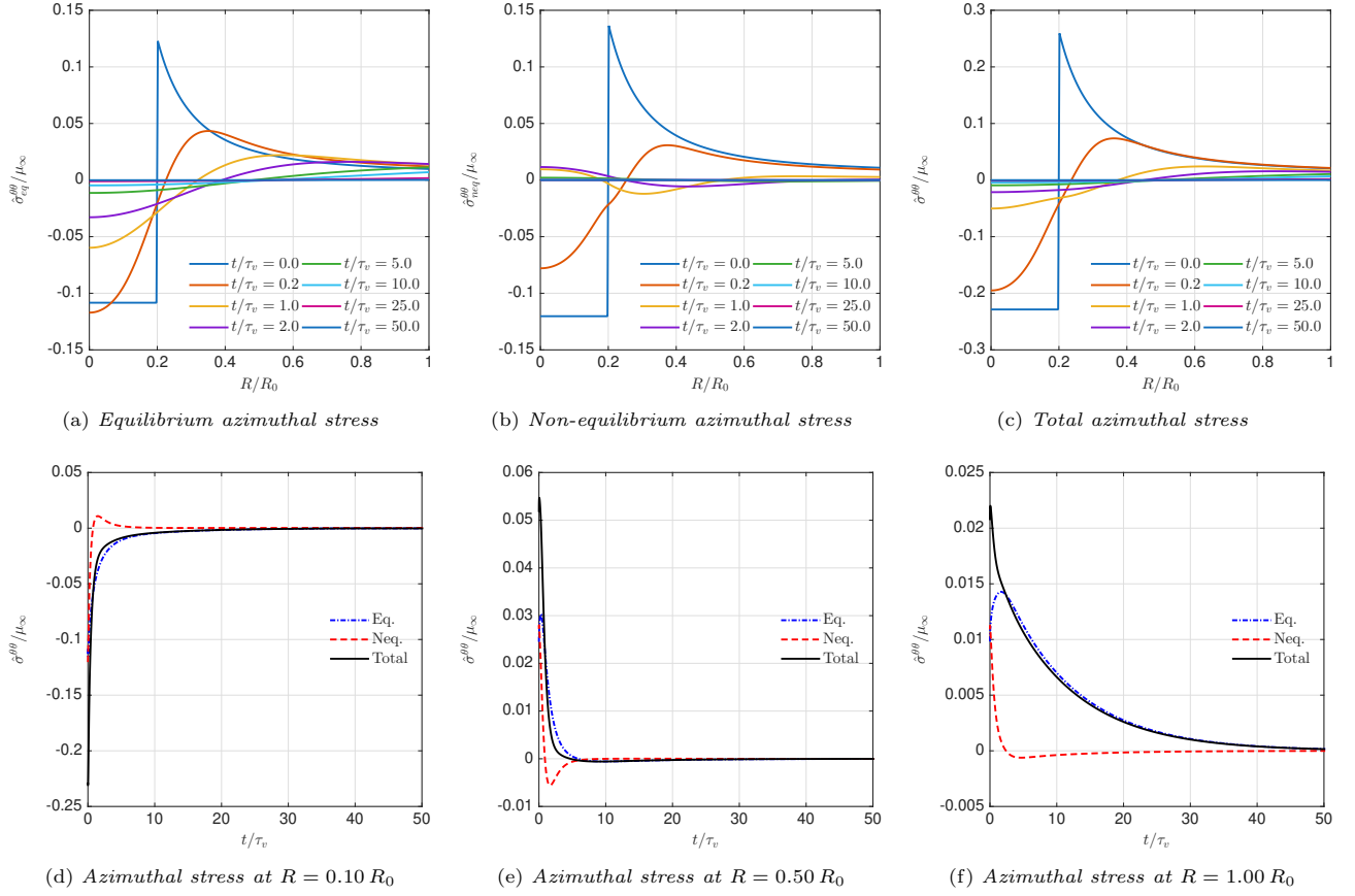
Figure 11: Azimuthal stress. Top row: spatial profiles at selected times. Bottom row: time evolution at fixed material radii.
