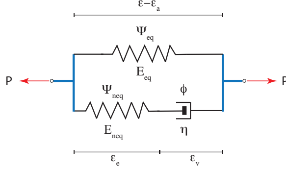
Figure 3: Standard anelastic solid: \Psi_{eq} , \Psi_{neq} , and \phi are the nonlinear analogues of E_{eq} , E_{neq} , and \eta , respectively. The total strain is decomposed as \varepsilon = \varepsilon_a + \varepsilon_e + \varepsilon_v , or equivalently \varepsilon - \varepsilon_a = \varepsilon_e + \varepsilon_v , where \varepsilon_e denotes the linearized elastic distortion, \varepsilon_v denotes the linearized viscous distortion, and \varepsilon_a denotes the linearized anelastic distortion. This additive decomposition is the linearization of any of the six possible multiplicative decompositions of the deformation gradient into elastic, anelastic, and viscous distortions, including the decomposition used in this paper, namely \mathbf{F} = \tilde{\mathbf{F}}\mathbf{F}^v\mathbf{F}^a .
