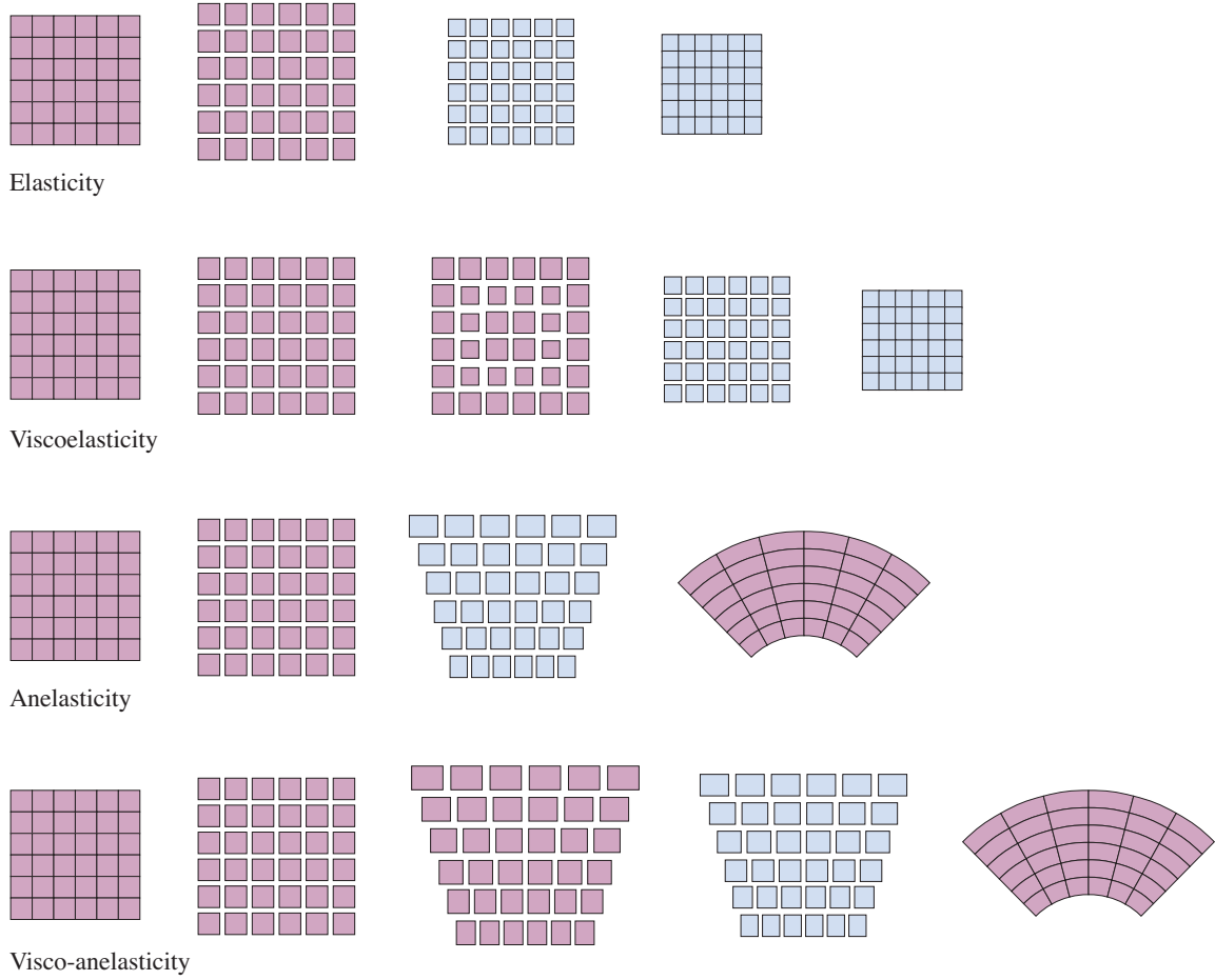
Figure 2: Schematic illustration of the elastic, viscoelastic, anelastic, and visco-anelastic responses of a sheet, illustrating the relation between local relaxation, compatibility, and the emergence of residual stress. Blue and pink indicate locally stress-free and locally stressed states, respectively.
