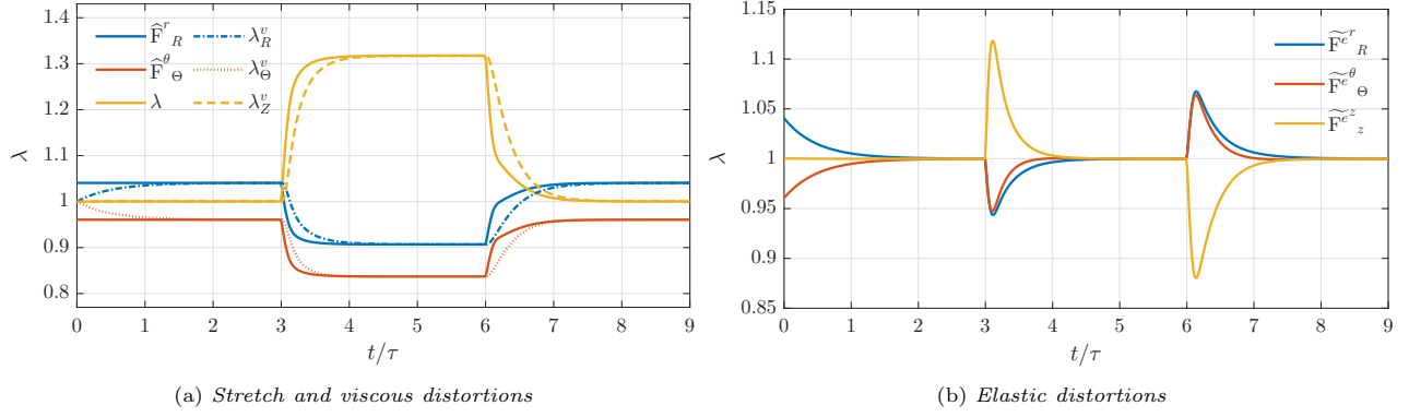
Figure 17: Force-controlled loading: evolution of the kinematics.
