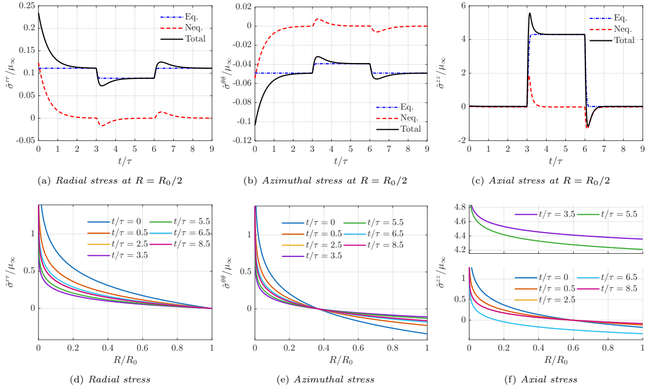
Figure 16: Displacement-controlled loading: stress evolution at fixed radius and stress radial profiles.
