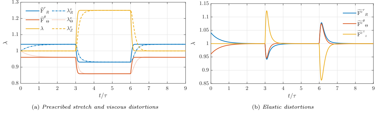
Figure 14: Displacement-controlled loading: evolution of the kinematics.
