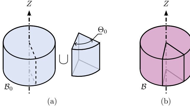
Figure 13: (a) A negative wedge disclination of magnitude \Theta_0 is constructed by making an axial cut in the stress-free cylinder B_0 and inserting into the cut a wedge of the same material with opening angle \Theta_0 . (b) The resulting body B containing a single wedge disclination in its stressed configuration.
