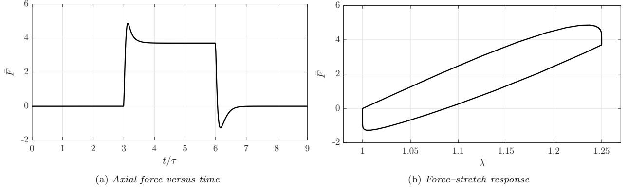
Figure 15: Displacement-controlled loading: global force response against time and axial stretch.
