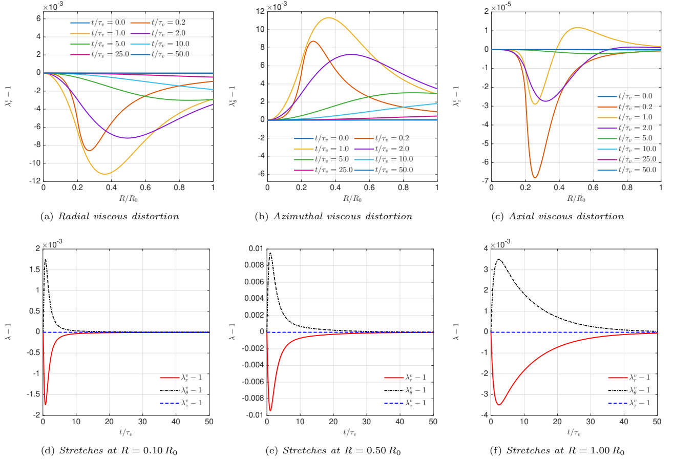
Figure 8: Viscous stretches. Top row: spatial profiles at selected times. Bottom row: time evolution at fixed material radii.
