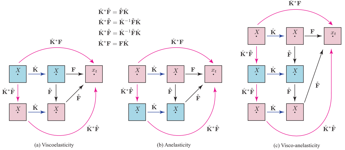
Figure 4: The actions of the symmetry group on the total, viscous, elastic, and anelastic deformation gradients. The blue and pink squares indicate locally stress-free and locally stressed configurations, respectively.
