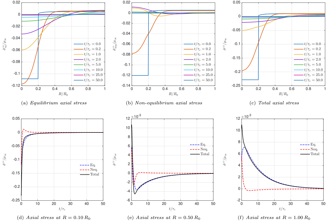
Figure 12: Axial stress. Top row: spatial profiles at selected times. Bottom row: time evolution at fixed material radii.
