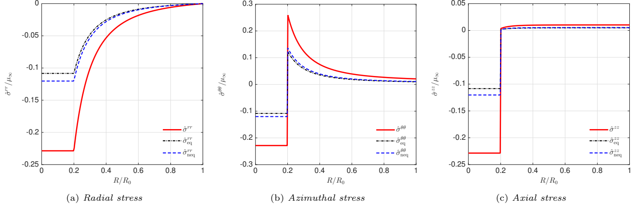
Figure 9: Snapshot of stresses at t/\tau_v = 0 .
