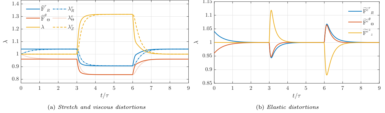
Figure 17: Force-controlled loading: evolution of the kinematics.
