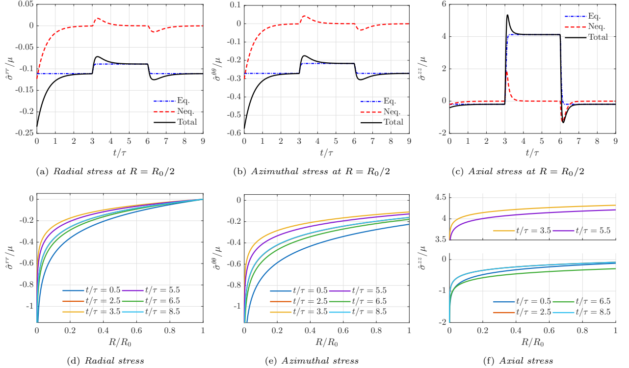
Figure 16: Displacement-controlled loading: stress evolution at fixed radius and stress radial profiles.
