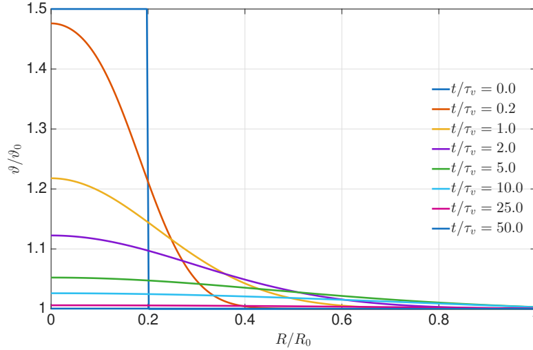
Figure 6: Temperature field \vartheta(R, t) at selected times.
