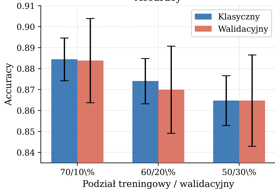
Accuracy
