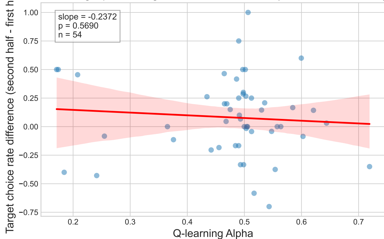
Q-learning Alpha vs Target choice rate difference (second half - first half)
