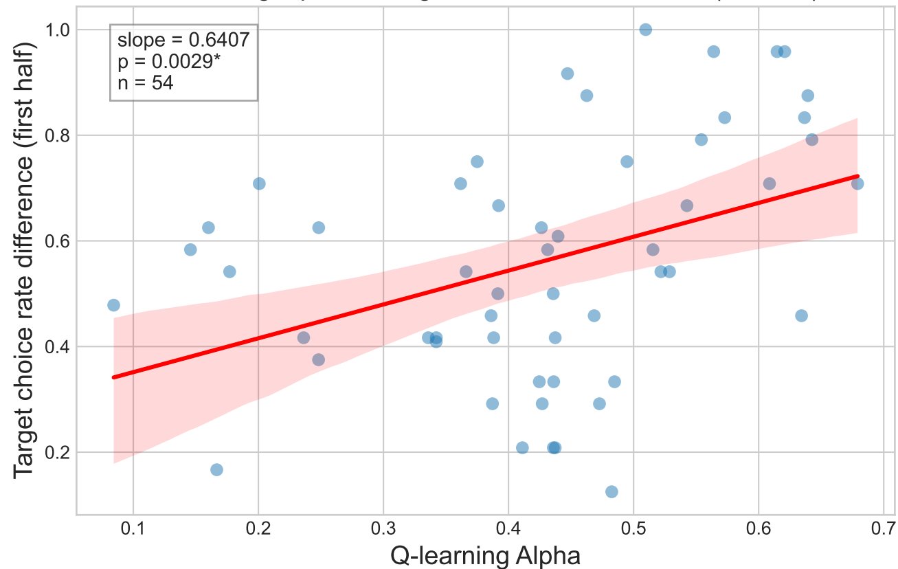
Q-learning Alpha vs Target choice rate difference (first half)
