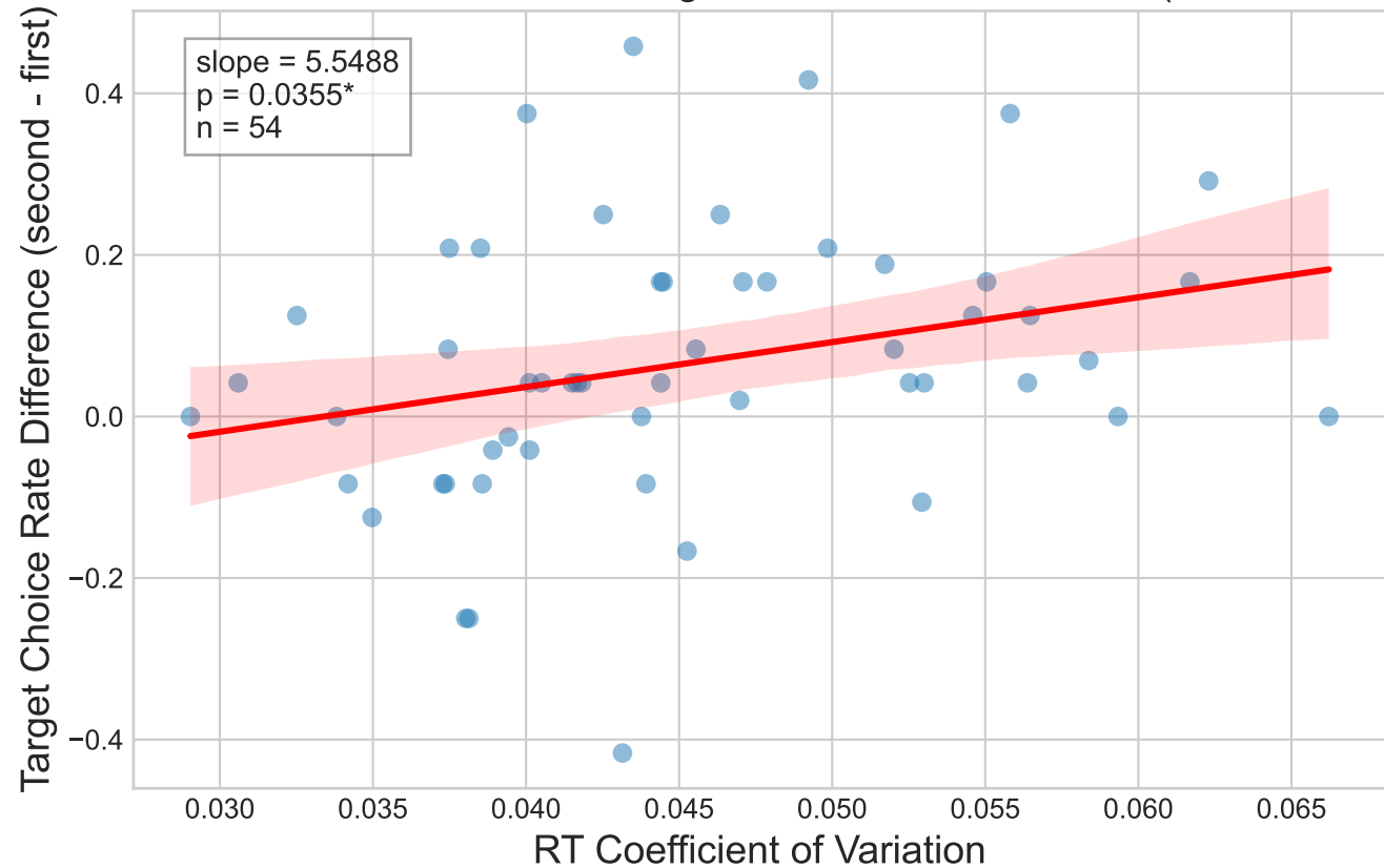
RT Coefficient of Variation vs Target Choice Rate Difference (second - first)
