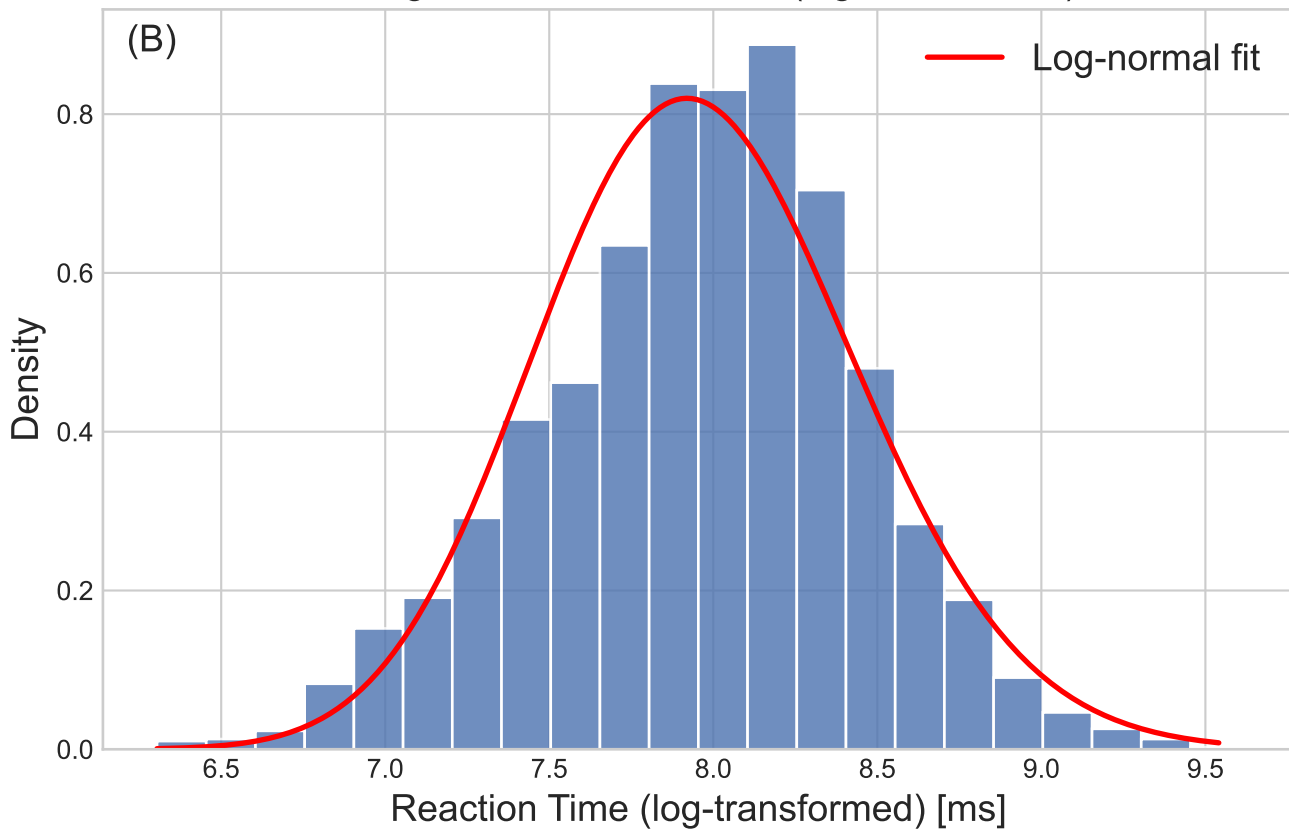
Histogram of Reaction Time (log-transformed)
