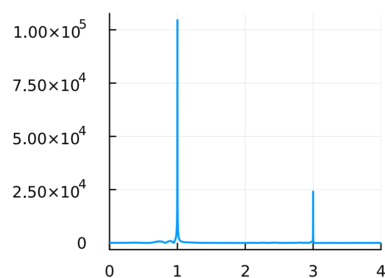
F=1.5, \omega=1.0
