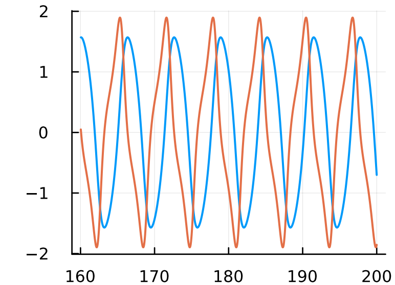
F=1.5, \omega=1.0
