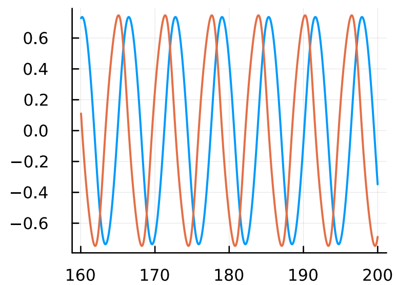
F=0.5, \omega=1.0
