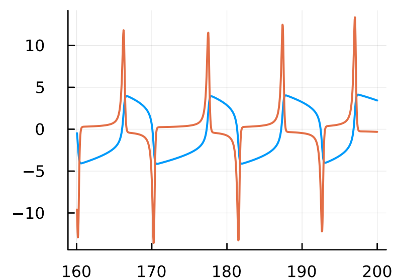
F=1.5, \omega=0.1
