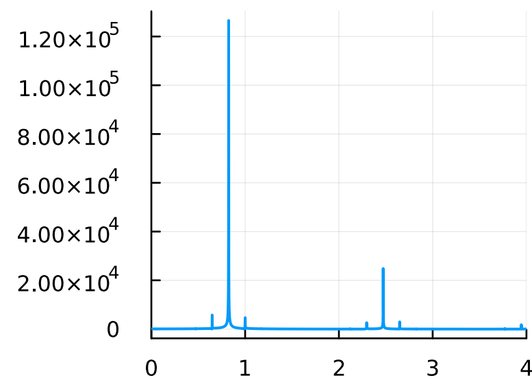
F=0.5, \omega=1.0
