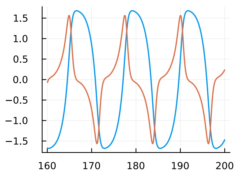
F=1.5, \omega=0.5
