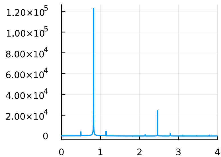
F=0.5, \omega=0.5
