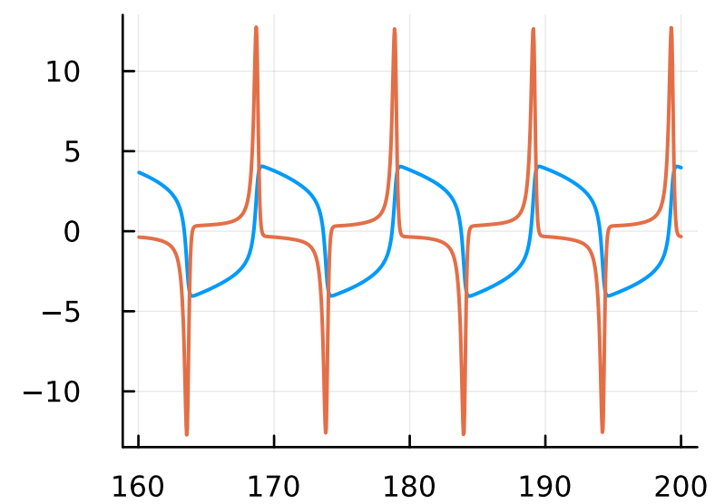
F=0.5, \omega=1.5
