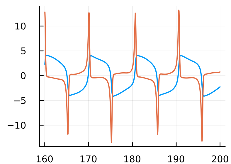
F=1.5, \omega=1.5
