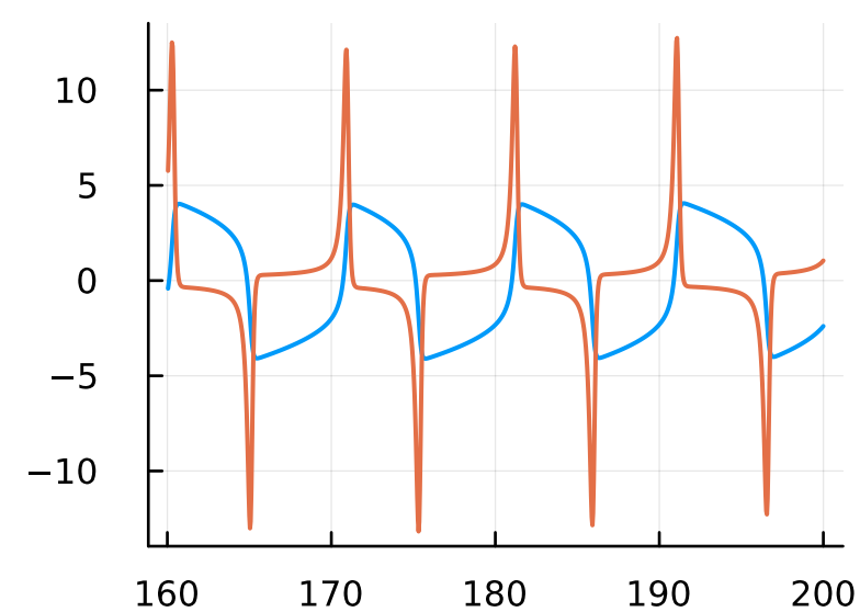
F=1.0, \omega=0.1
