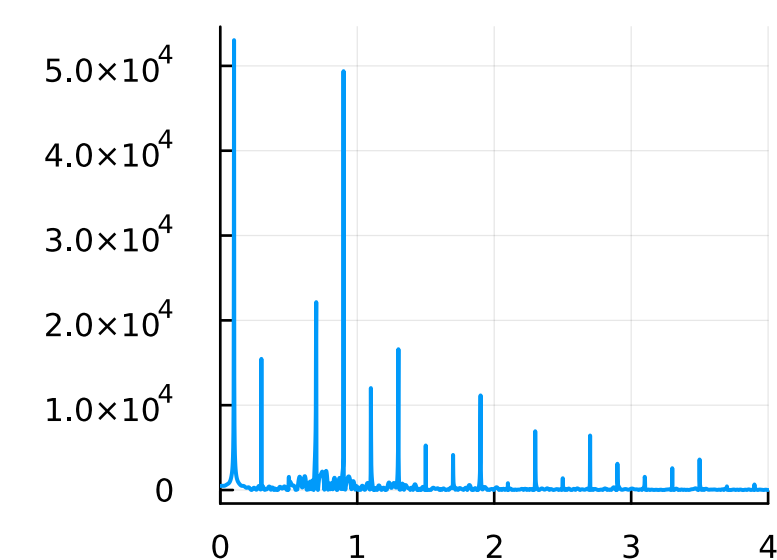
F=1.5, \omega=0.1
