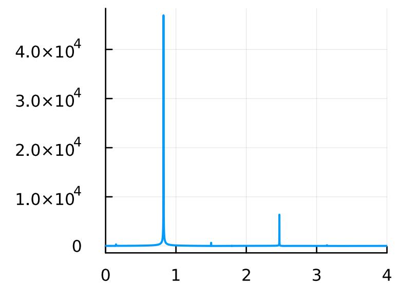
F=0.5, \omega=1.5
