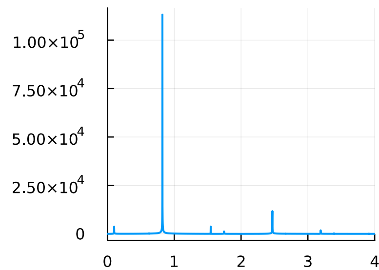
F=0.5, \omega=0.1
