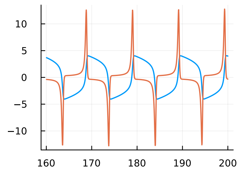
F=0.5, \omega=0.1
