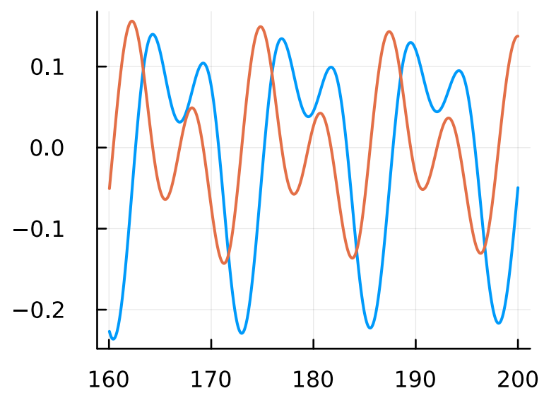
F=0.5, \omega=0.5
