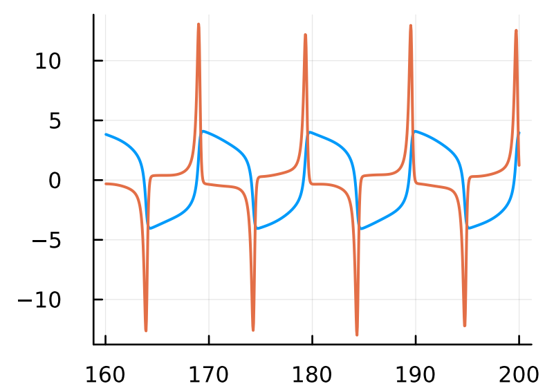
F=1.0, \omega=1.5
