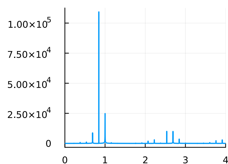
F=1.0, \omega=1.0
