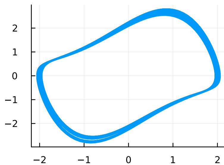
F=0.5, \omega=0.5
