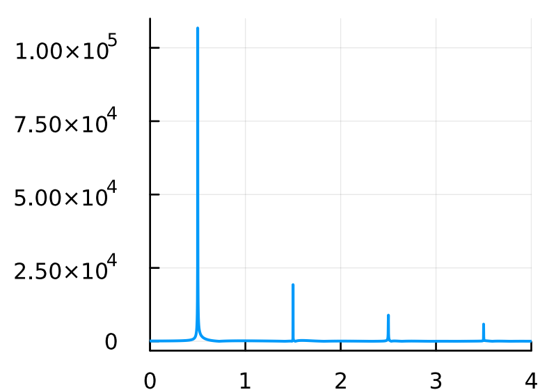
F=1.5, \omega=0.5
