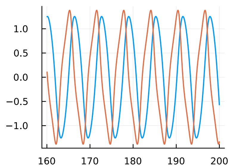
F=1.0, \omega=1.0
