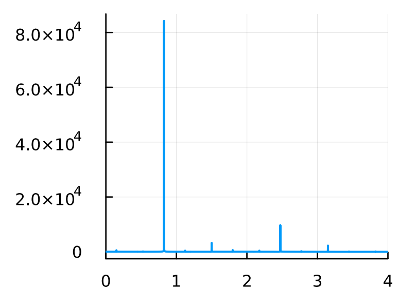
F=1.0, \omega=1.5
