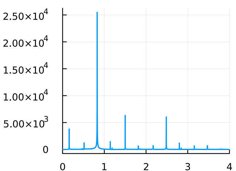
F=1.5, \omega=1.5
