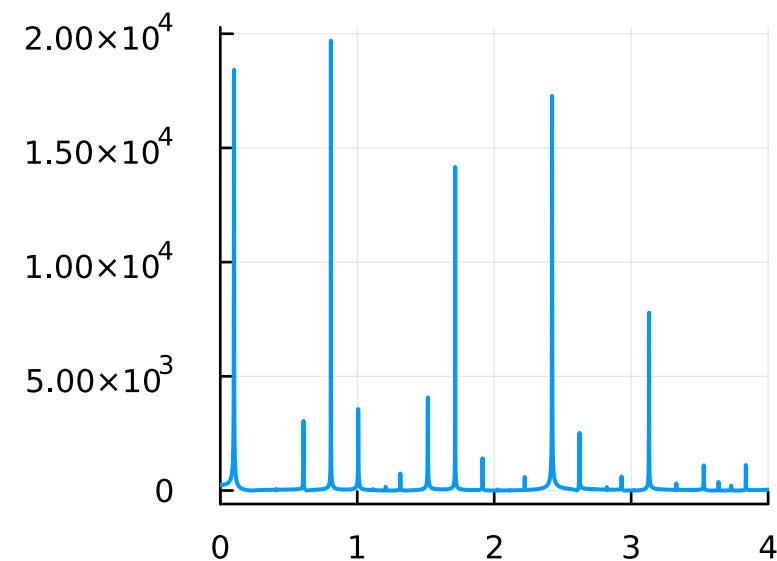
F=1.0, \omega=0.1
