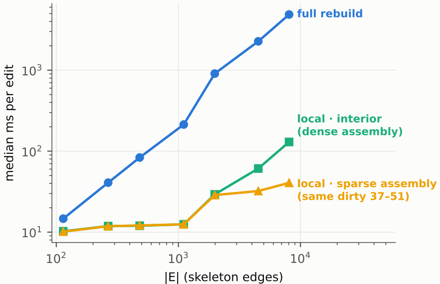
Per-edit rebuild cost (log-log)
