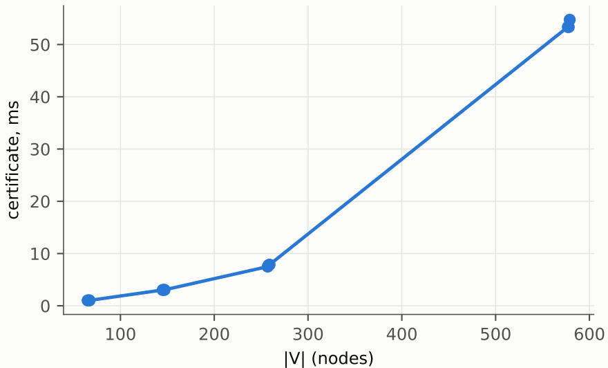
Mayer-Vietoris certificate cost
