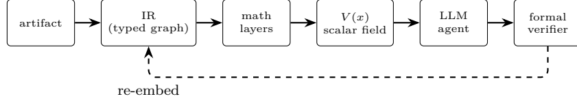
Figure 1: The pipeline: an artifact becomes a typed graph, enriched with mathematical structure into a vulnerability scalar field V(x) , which an LLM agent navigates; a formal verifier confirms or refutes each hypothesis and the result re-embeds into the manifold.
