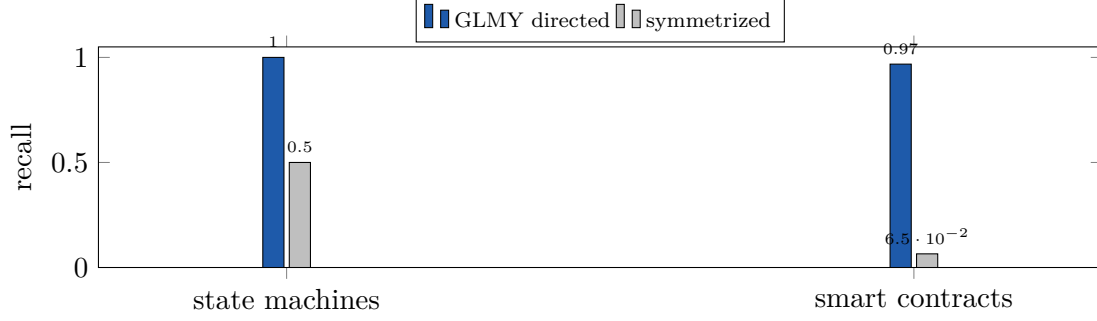
Figure 3: Directed (GLMY) path homology vs. symmetrized homology for destructive cycle detection. Symmetrization collapses the directed 2-cycle — recall drops from 1.0 to 0.5 on state machines and from 0.97 to 0.065 on smart contracts.
