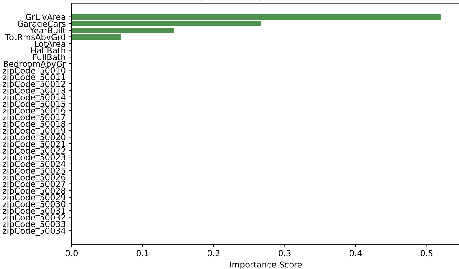
Feature Importance (zipCode One-Hot Encoded)
