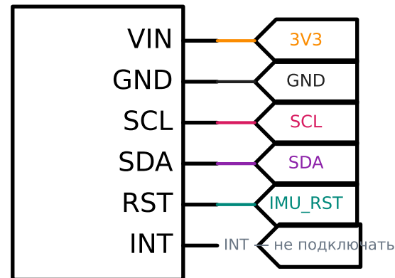
IMU BNO085 (Game Rotation Vector)
