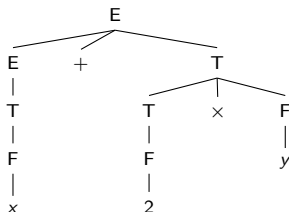
Derivation/parse tree
