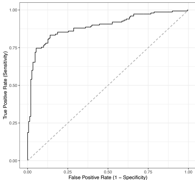
ROC Curve for Logistic Regression
