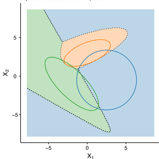
Theoretical Bayes Classifier (QDA)
