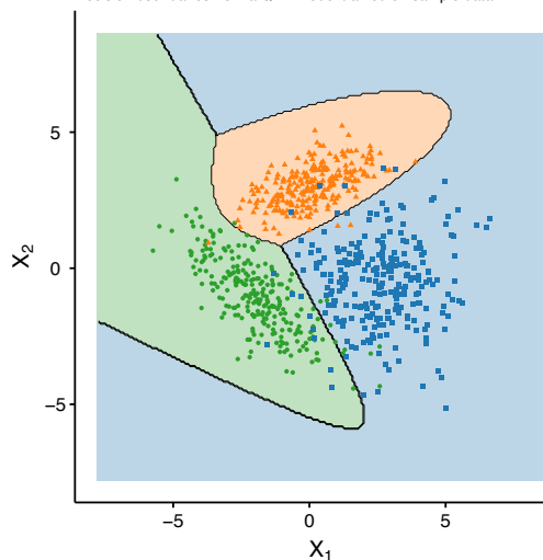
Quadratic Discriminant Analysis
