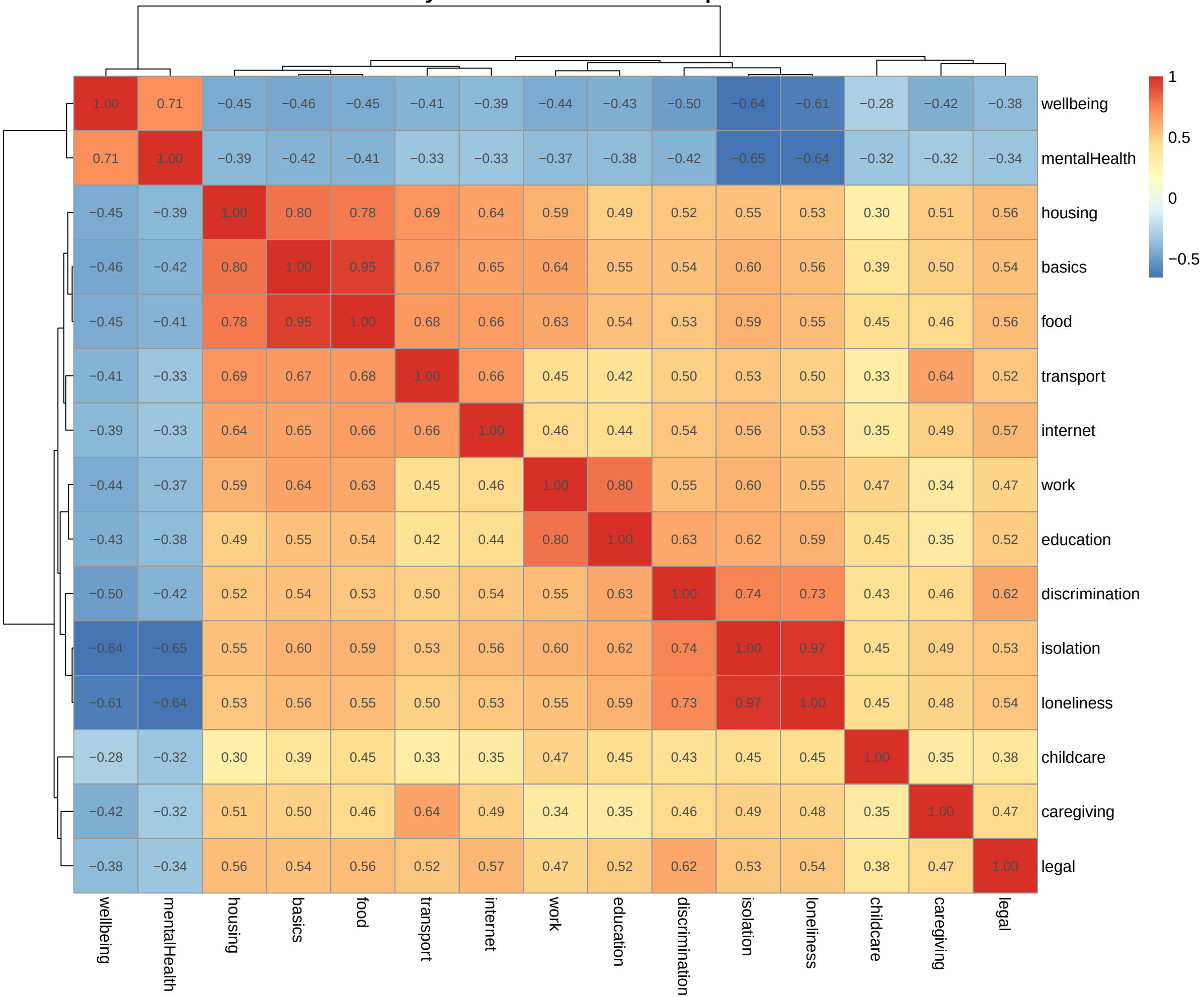
Polychoric Correlation Heatmap
