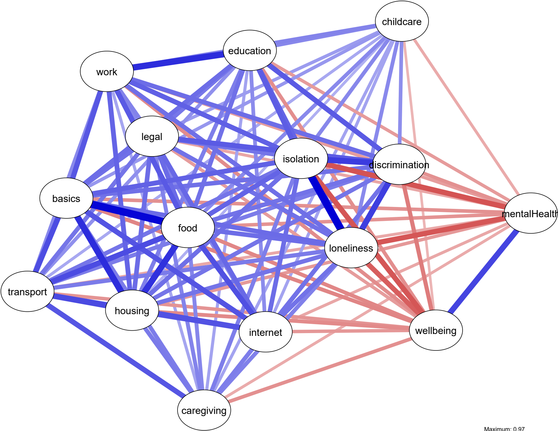
Correlation Network (no trimming)
