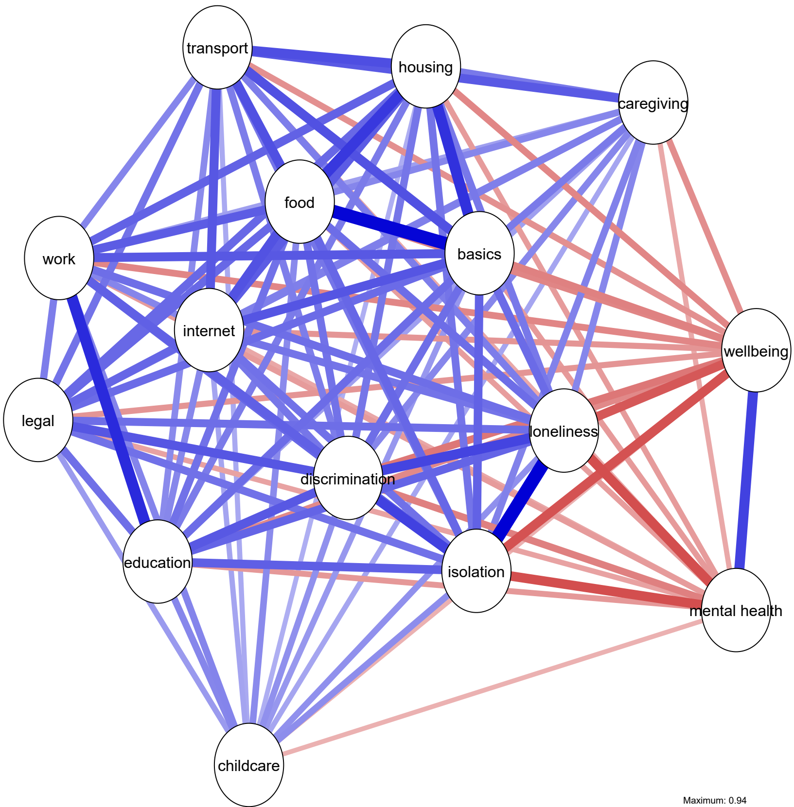
Correlation Network of outcomes with needs (no trimming)
