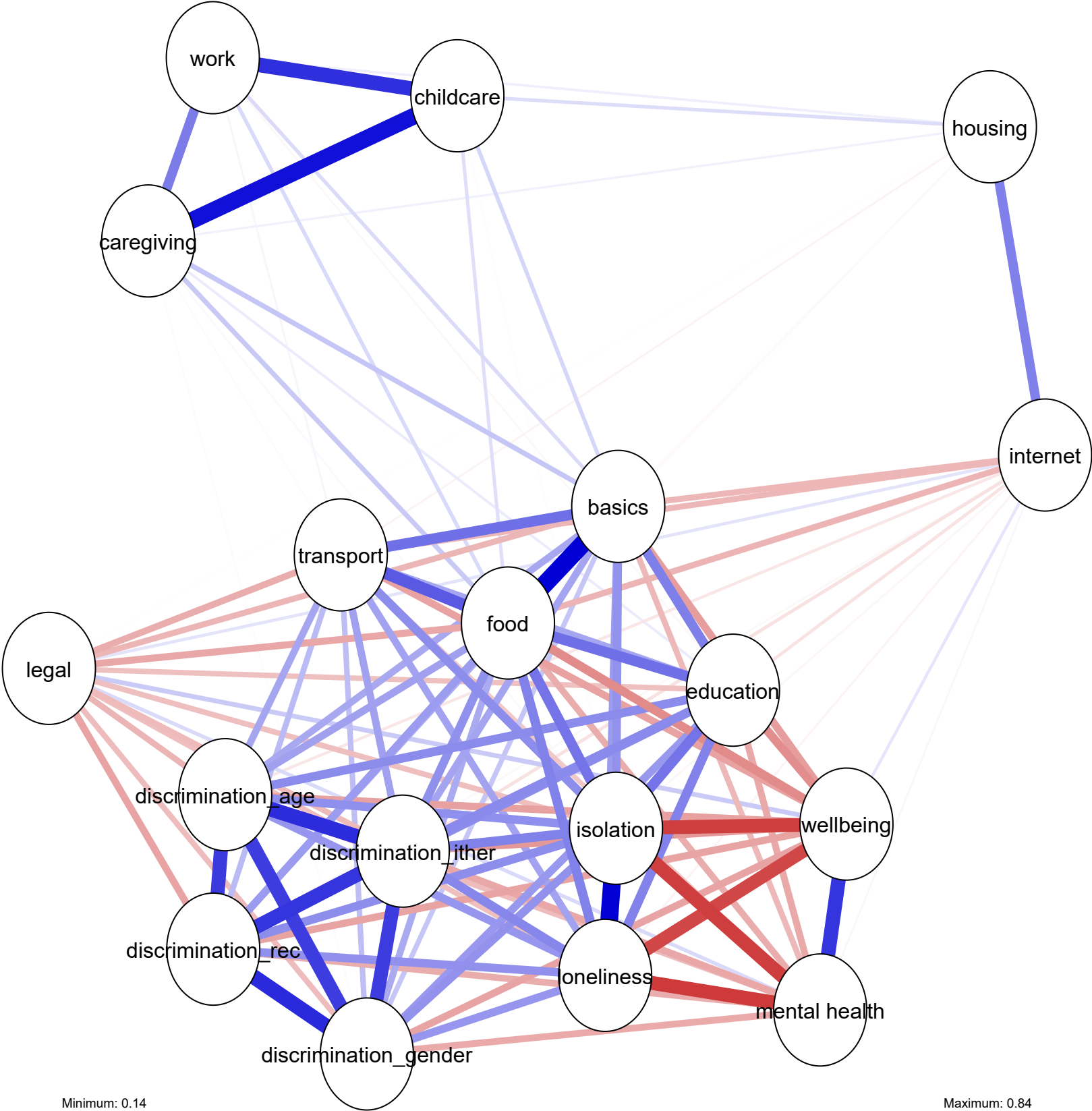
Correlation Network (trimming 1/2 of edges)
