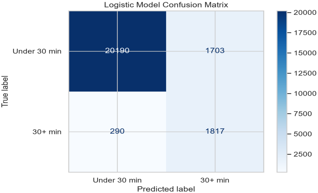
Figure 3. Balanced logistic regression confusion matrix.
