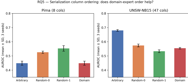
Fig. 3. Mean AUROC by serialization column ordering on pima and UNSW-NB15 (Qwen2.5-3B prompted, 3 seeds per condition).
