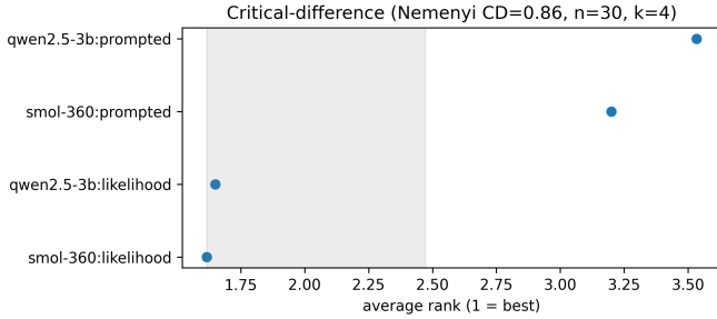
Fig. 1. Critical-difference diagram for four conditions on 30 ODDS datasets (Friedman p = 6.0 \times 10^{-12} ). Connected conditions are not significantly different by Nemenyi post-hoc test.
