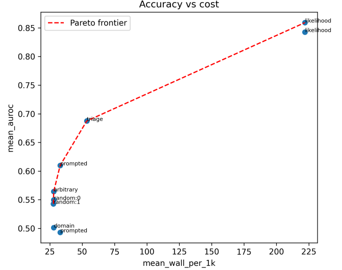
Fig. 4. Mean AUROC vs. wall time per 1,000 test rows for tested LLM and classical scoring modes.
