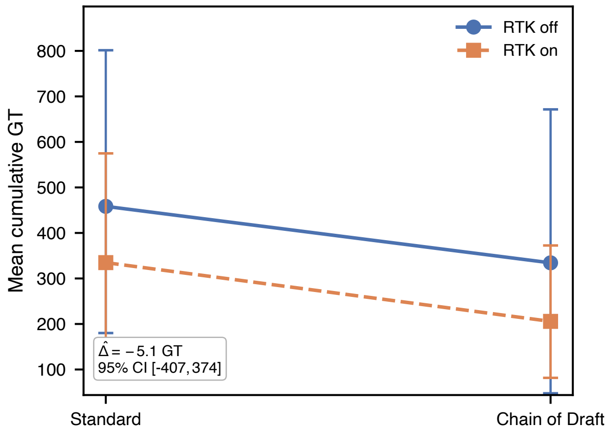
Figure 5: Mean cumulative GT per cell, E2 (RTK-CoD) experiment ( n = 36 ). Error bars show run-level bootstrap confidence intervals for individual cell means; the interaction interval uses the preregistered task-seed block bootstrap. Solid/dashed lines: RTK off/on. Interaction \hat{\Delta} = -5.06 \text{ GT} (95% CI [-407, +374]). Observed marginal differences: RTK \approx -124 \text{ GT} ; CoD \approx -126 \text{ GT} (descriptive contrasts; no CIs).
