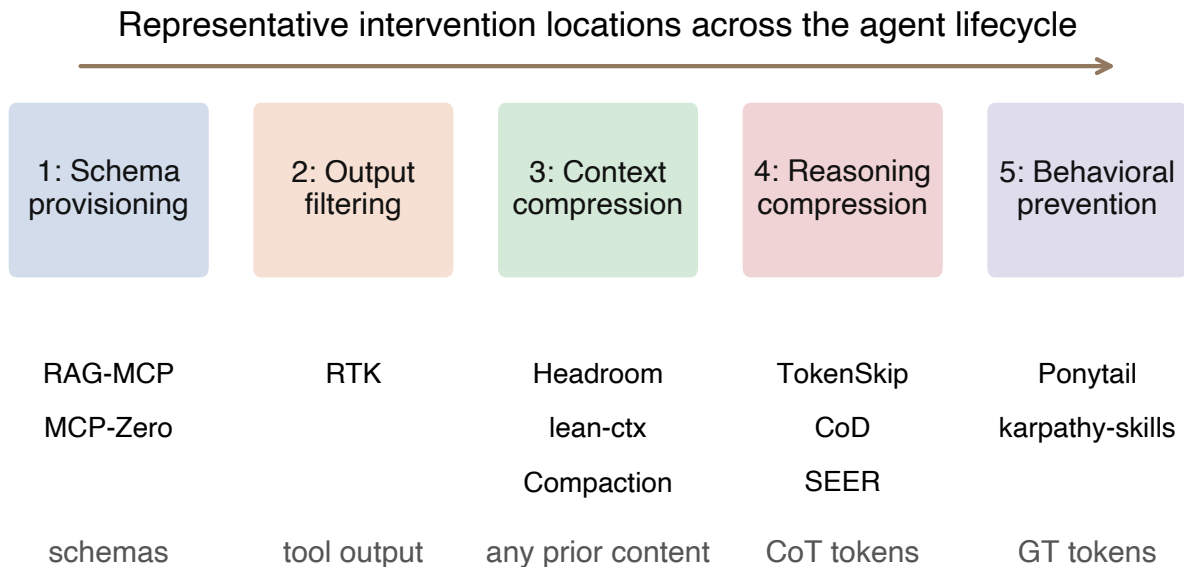
Figure 2: Schematic of five intervention points in the agent token lifecycle, with representative methods per category (not exhaustive; Table 1 lists all sixteen). Labels below each category denote token populations; the arrow indicates representative intervention locations across the lifecycle, not a mandatory sequential pipeline.
