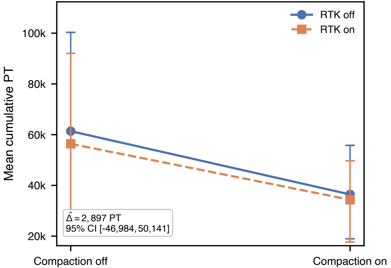
Figure 4: Mean cumulative PT per cell, E1 (RTK-compaction) experiment ( n = 12 ). Error bars show run-level bootstrap confidence intervals for individual cell means; the interaction interval uses the preregistered task-seed block bootstrap. Solid circles/blue: RTK off; dashed squares/orange: RTK on. Interaction \hat{\Delta} = +2,897 PT (95% CI [−46,984, +50,141]).
