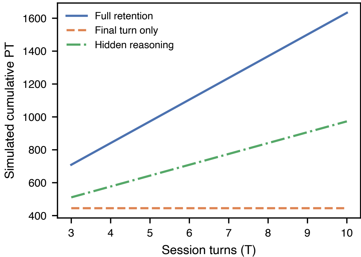
Figure 3: Simulated cumulative prompt tokens under a TokenSkip-like compression profile (313→181 generated tokens per reasoning step, \gamma=0.42 ; based on published aggregate values from TokenSkip, not a reproduced run) across session lengths T . Full retention : saved reasoning re-enters every later prompt. Final turn only : the saving appears only in the final response. Hidden reasoning : reasoning never enters subsequent prompts. Counterfactual illustration derived from (7), not an experimental result.
