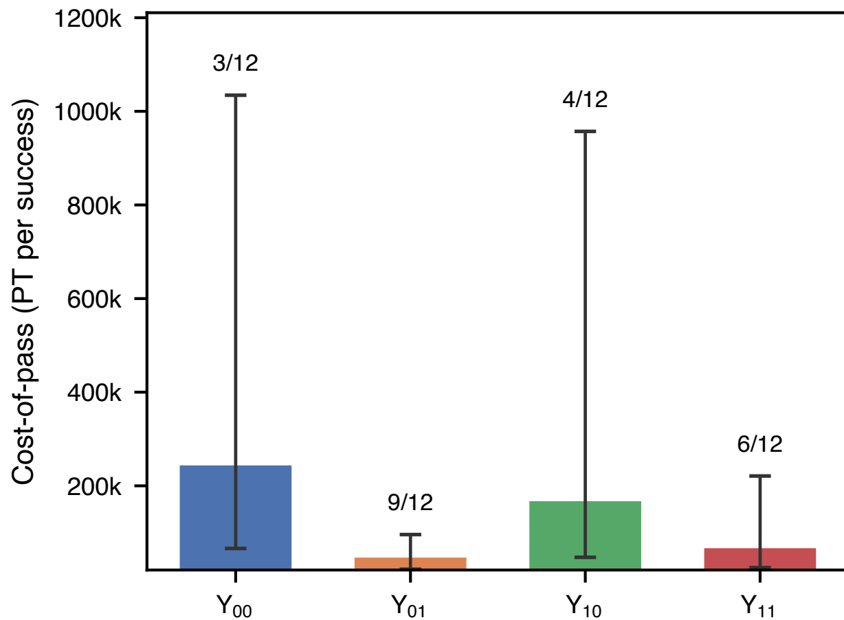
Figure 6: Cost-of-pass (Erol et al., 2025) (prompt tokens per successful task completion) by treatment cell, E1 experiment. Error bars show run-level bootstrap intervals for descriptive estimates; bootstrap replicates with zero successful runs were undefined and omitted. Success counts are shown above each bar. Descriptive secondary analysis, not a preregistered confirmatory result.
