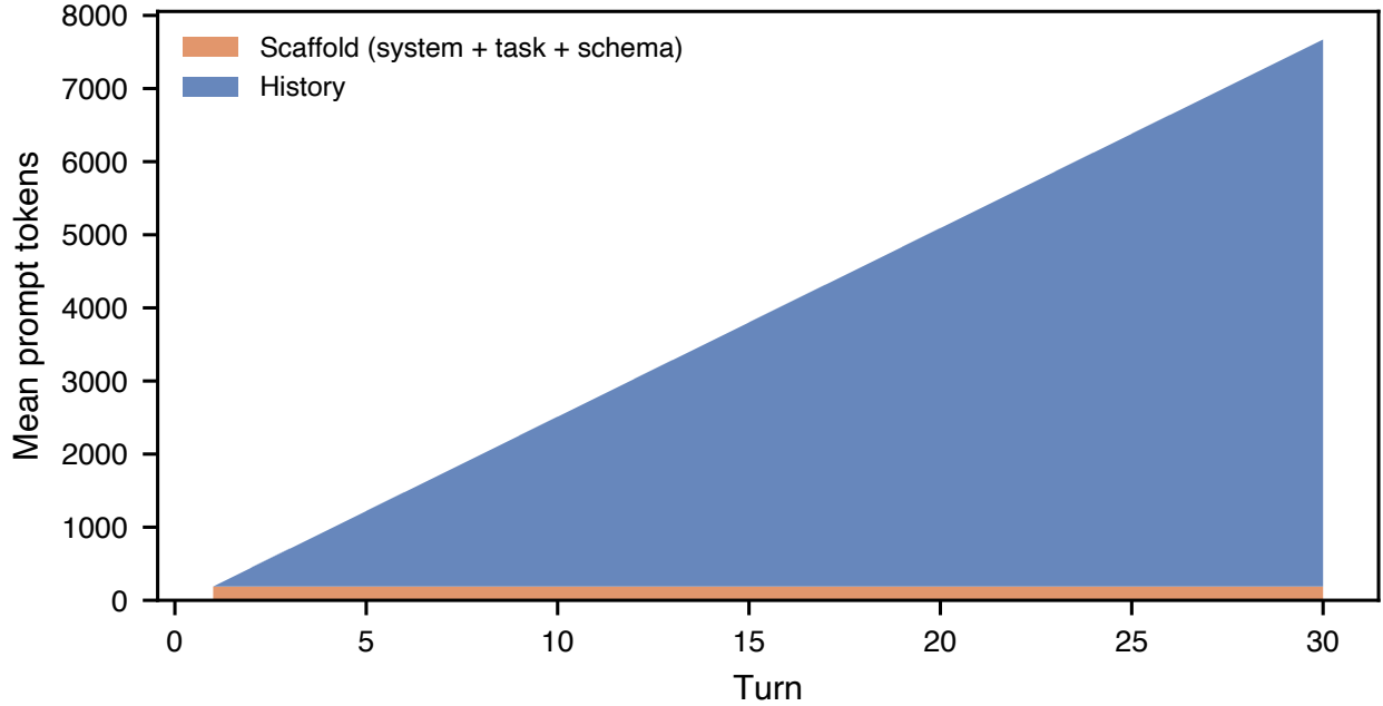
Figure 1: Stacked mean prompt tokens by region across agent turns (RTK off, compaction off, n = 12 runs). Scaffold (system, task, and tool schema) is constant at 189 tokens; history accumulates above it at a mean rate of 258 tokens per turn.
