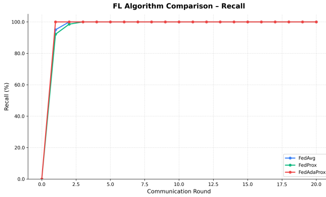
Fig. 9. Recall on N-BaIoT over 20 communication rounds.
