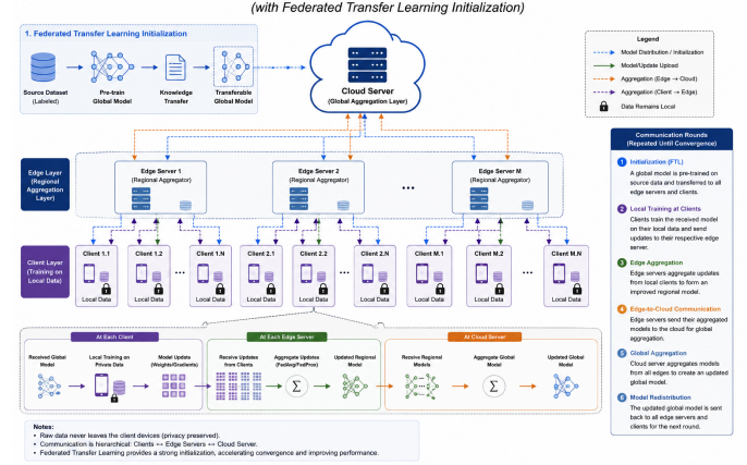
Fig. 2. Hierarchical Federated Communication Workflow: FTL initialization phase (once) followed by the six-stage per-round federated optimization phase.
