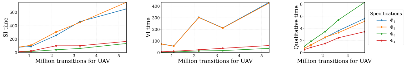
Fig. 13: Performance comparison for the UAV benchmarks under the selected GR(1) specifications. The columns correspond to Strategy Improvement (left), Value Iteration (middle), and Qualitative Analysis (right). All times are reported in seconds. The legend is shown only once; the same color-to-specification mapping is used across all subfigures.
