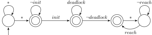
Fig. 9: GR(1)₁: \mathbf{GF}(init) \wedge \mathbf{GF}(\neg d) \rightarrow \mathbf{GF}(r) .
