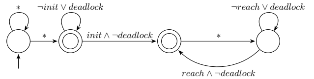
Fig. 12: GR(1)₄: \mathbf{GF}(init \wedge \neg d) \rightarrow \mathbf{GF}(r \wedge \neg d) .
