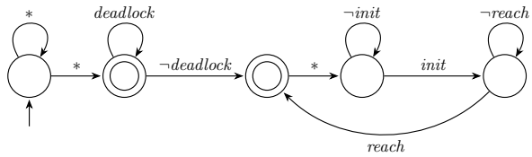
Fig. 10: GR(1)₂: \mathbf{GF}(\neg d) \rightarrow \mathbf{GF}(r) \wedge \mathbf{GF}(init) .
