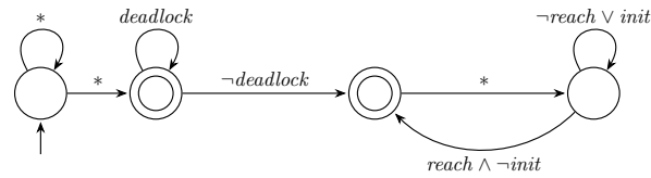
Fig. 11: GR(1)₃: \mathbf{GF}(\neg d) \rightarrow \mathbf{GF}(r \wedge \neg init) .
