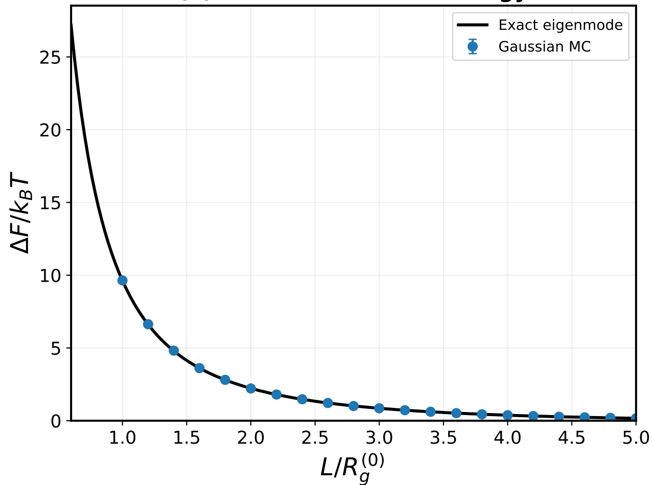
(a) Confinement free energy
