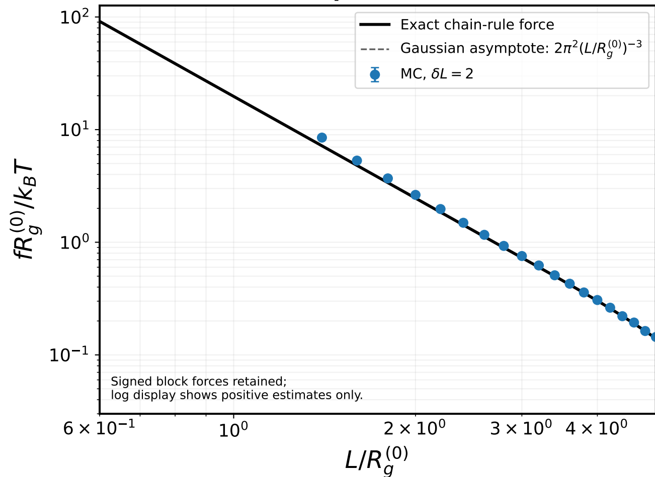
(b) Entropic force ( \delta L = 2 )
