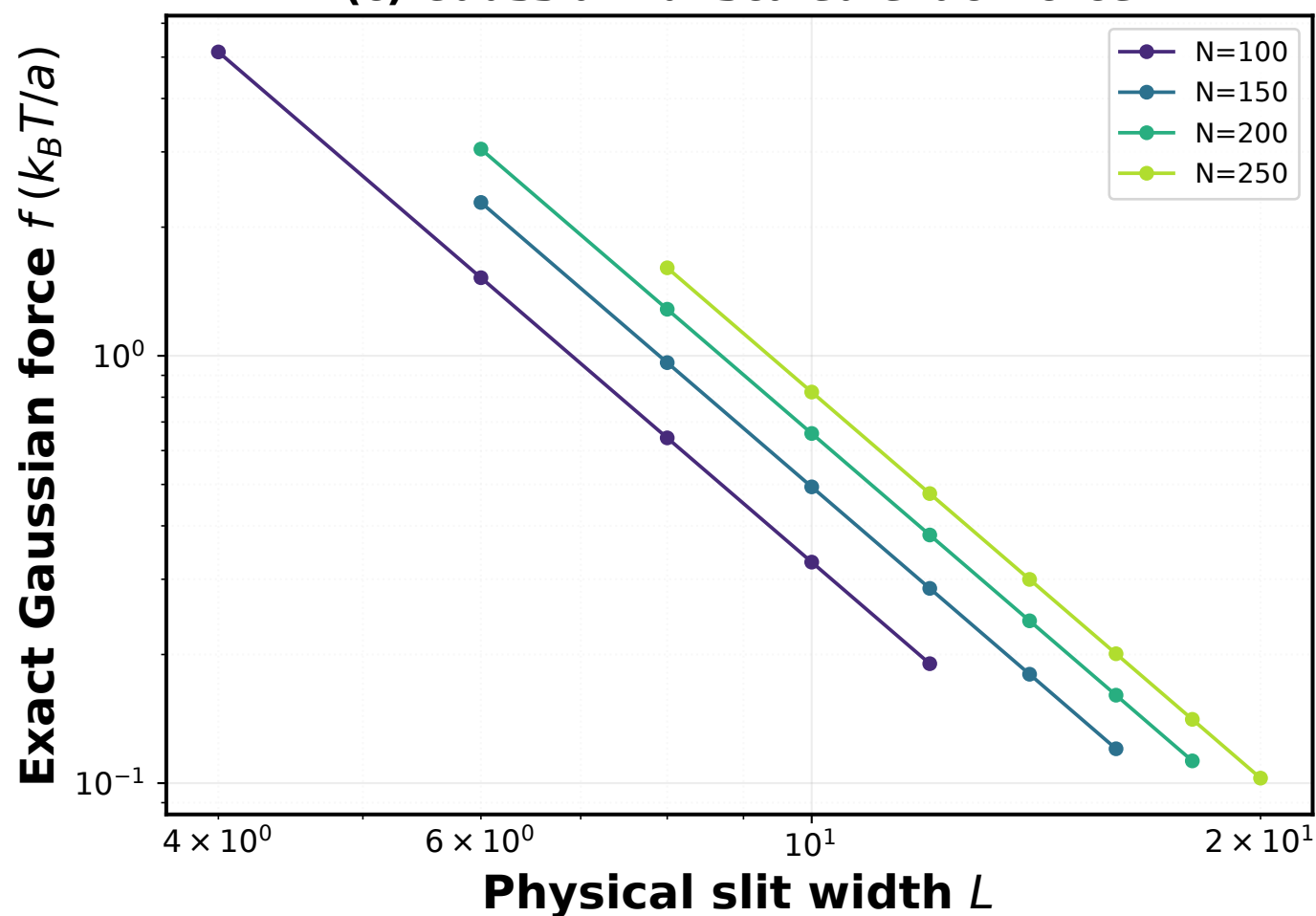
(c) Gaussian: unscaled exact force
