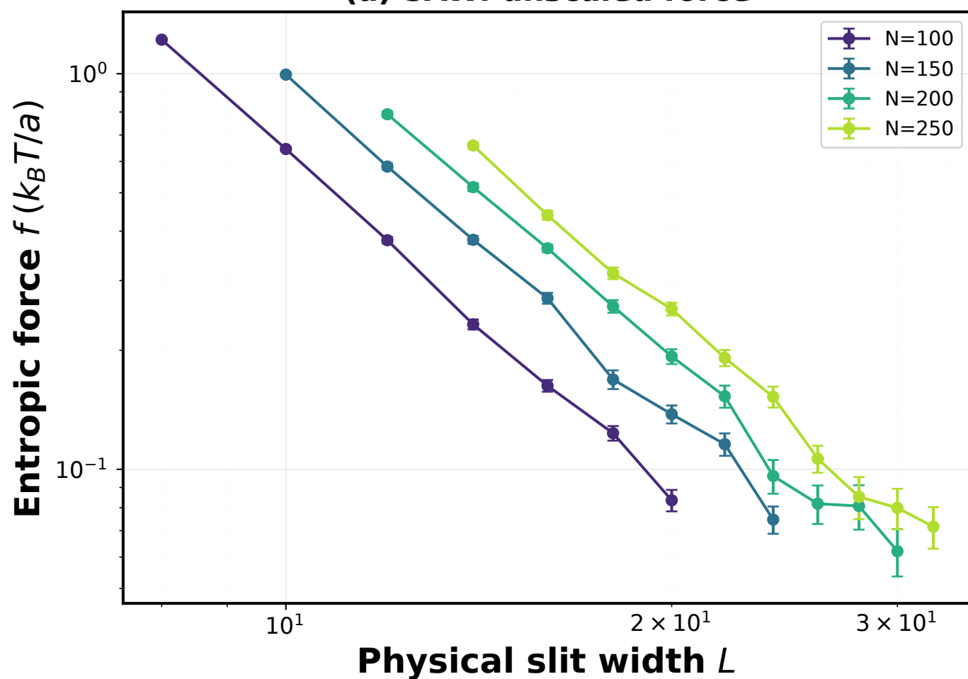
(a) SAW: unscaled force
