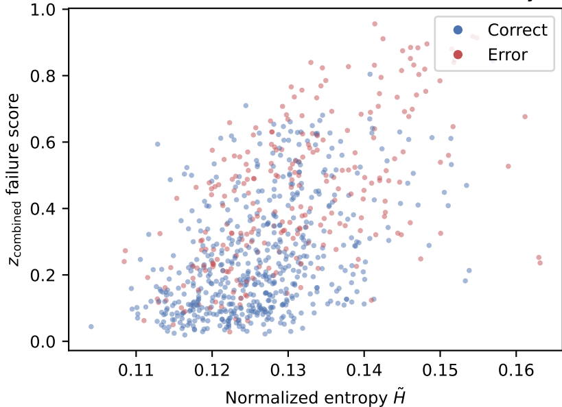
ID test (seed 42; subset; correctness memory)
