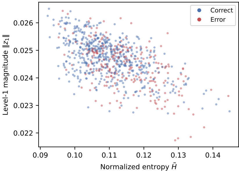
ID test (seed 42; subset shown)
