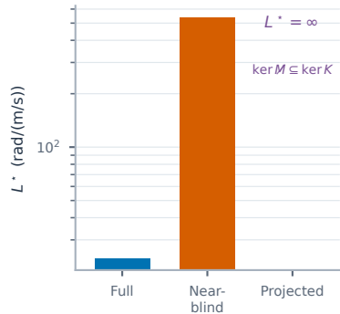
C Two failure modes
