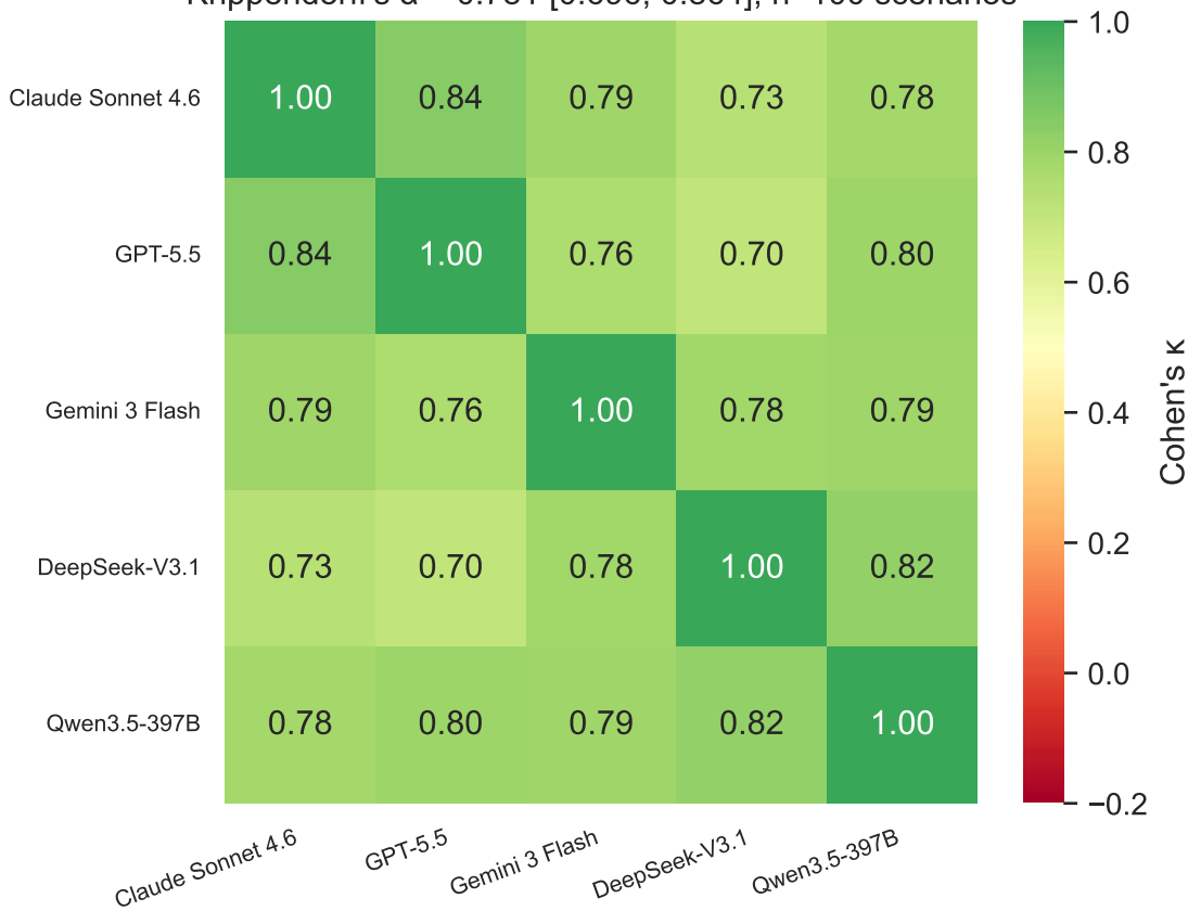
Pairwise binary-judgment agreement — Instant mode Krippendorff's \alpha = 0.781 [0.696, 0.864], n=100 scenarios
