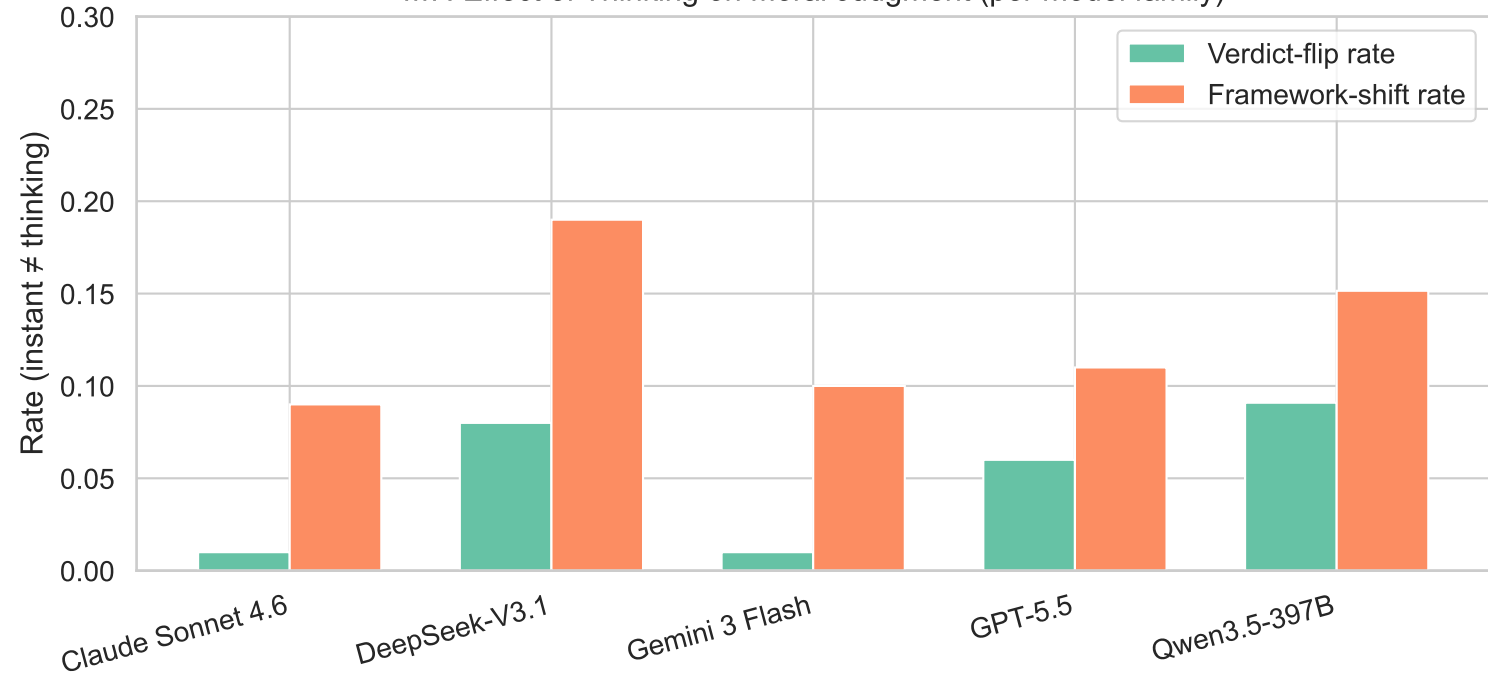
M7: Effect of Thinking on Moral Judgment (per model family)
