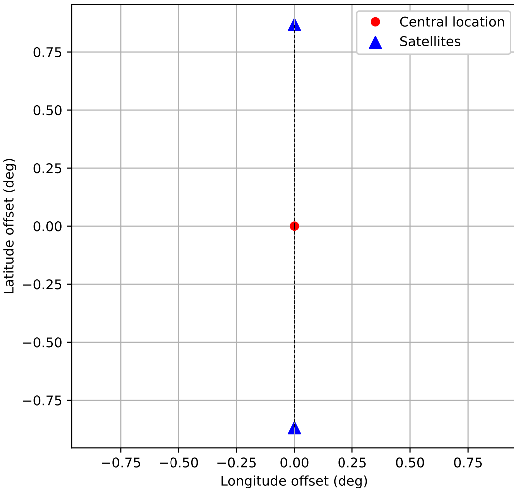
Symmetric Satellite Constellation at Epoch 2025-09-26 (H=600 km)
