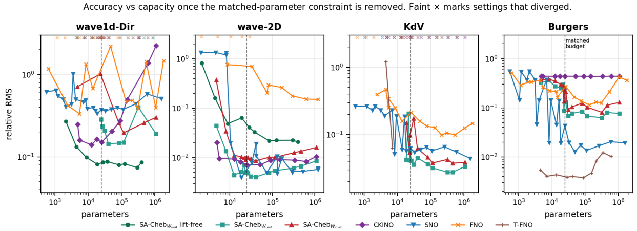
Figure 12: Accuracy against parameter count with the matched budget removed; the dashed line marks the 25k budget used in Table 5. The ranking is budget-dependent, so the matched table should be read as “best at 25k” rather than “best architecture”.
