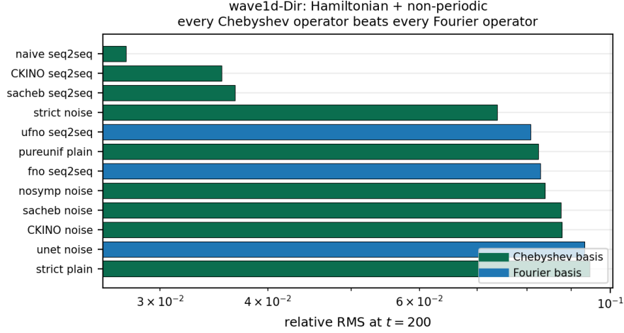
Figure 8: wave1d_dir , the Hamiltonian non-periodic rung. Every Chebyshev operator beats every Fourier operator: 3.0\times over the best FNO and 4.9\times over SNO, on a benchmark built to match SNO’s own data protocol. The mechanism is the Gibbs penalty the Dirichlet envelope imposes on a periodic basis.
