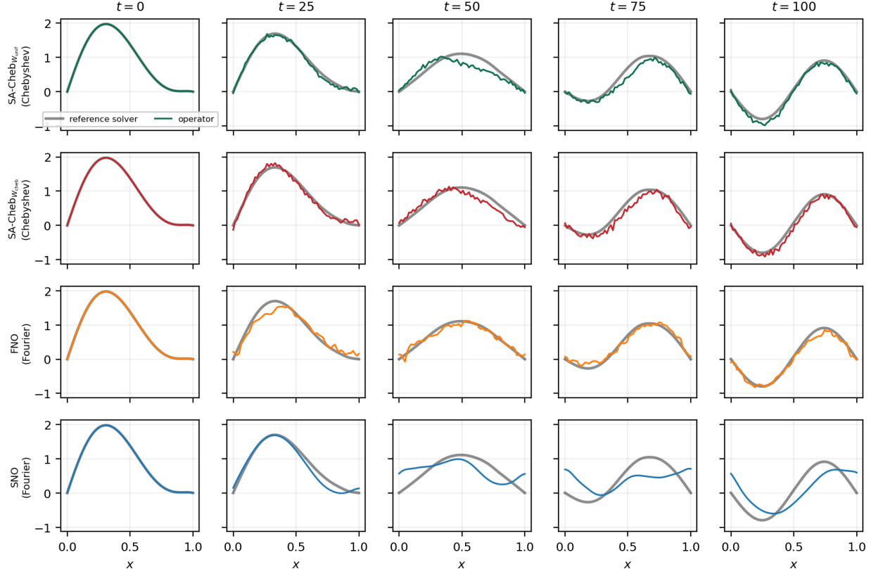
Figure 11: wave1d_dir : reference solver (grey) against operator prediction, displacement u(x, t) at five rollout times. The Chebyshev operators track the Dirichlet boundary; the Fourier operators accumulate the Gibbs error that Figure 8 quantifies. Reduced-schedule local reproduction, see §9.
