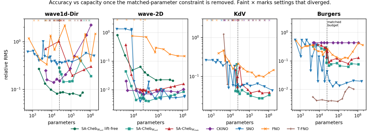
Figure 10: Accuracy against parameter count with the matched budget removed; the dashed line marks the 25k budget used in Table 4. The ranking is budget-dependent, so the matched table should be read as “best at 25k” rather than “best architecture”.
