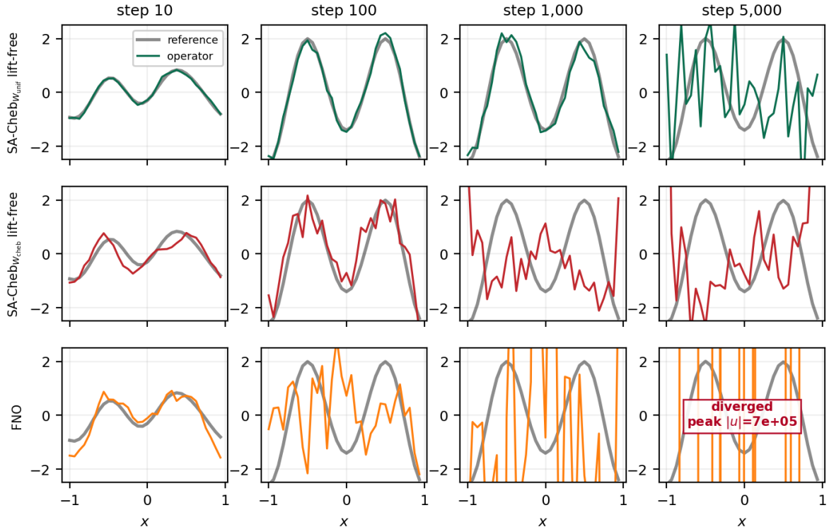
Figure 12: wave1d under long autoregressive rollout. The lift-free operators remain on the solution manifold at 5,000 steps while FNO has left it by 1,000. This is Figure 7 viewed as fields rather than curves. Reduced-schedule local reproduction, see §9.
