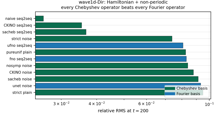
Figure 8: wave1d_dir , the Hamiltonian non-periodic rung. Every Chebyshev operator beats every Fourier operator: 3.2\times over the best FNO and 6.5\times over SNO, on a benchmark built to match SNO’s own data protocol. The mechanism is the Gibbs penalty the Dirichlet envelope imposes on a periodic basis.
