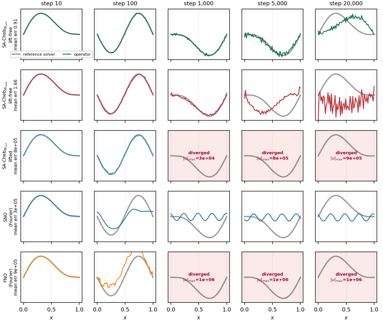
Figure 11: wave1d.dir time lapse over the 2 \times 10^4 -step rollout: reference solver (grey) against operator prediction. Row labels carry each family's population error over all test trajectories, so a single plotted trajectory cannot be over-read. Three distinct failure modes are visible and are not interchangeable: the lifted SA-Cheb and FNO blow up; SNO collapses to a low-amplitude oscillation—bounded, but carrying none of the physics; only the lift-free operators track the wave to 2 \times 10^4 steps.
