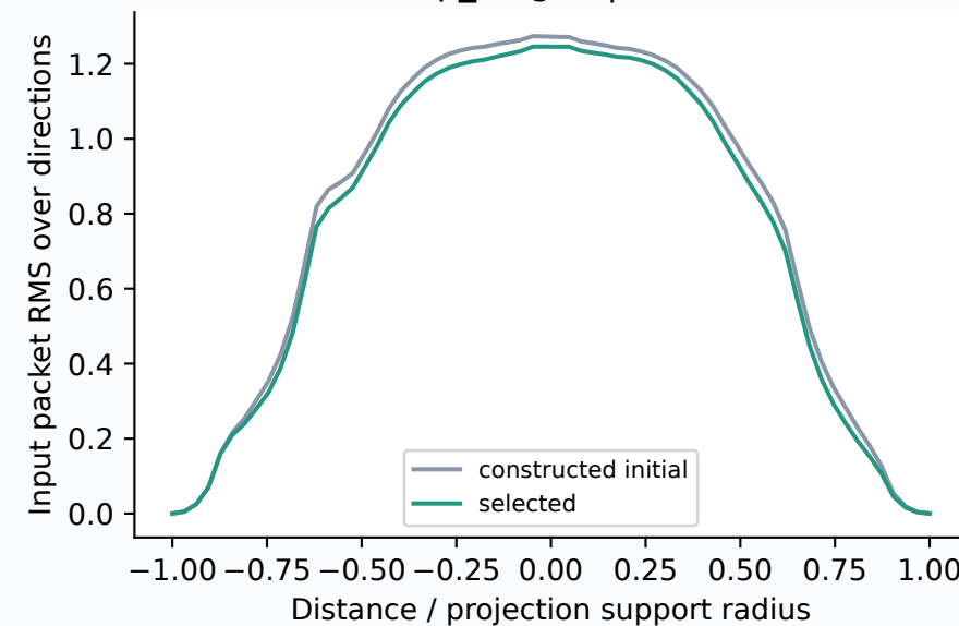
oct_stage3 | test
