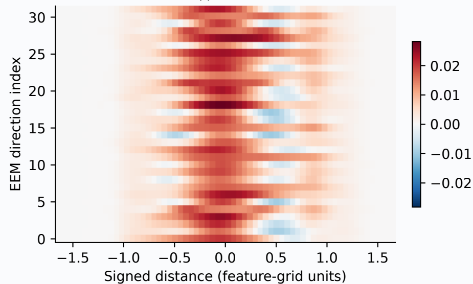
train | label1 minus label0 | cross_message_ms clipped 0.0%
