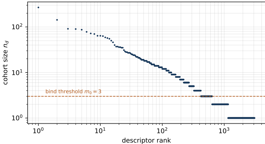
Moby-Dick descriptor cohorts (8631 sentences, 3078 descriptors)
