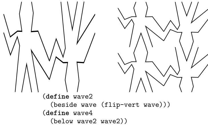
Figure 2.12 Creating a complex figure, starting from the wave painter of figure 2.10.
