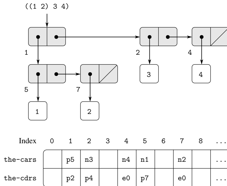
Figure 5.14 Box-and-pointer and memory-vector representations of the list ((1 2) 3 4) .
