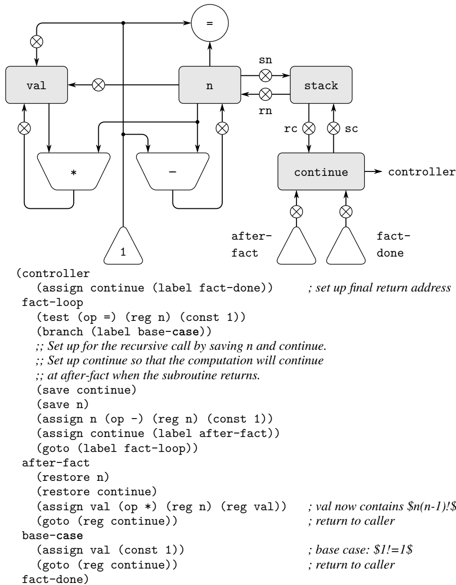
Figure 5.12 A recursive factorial machine.
