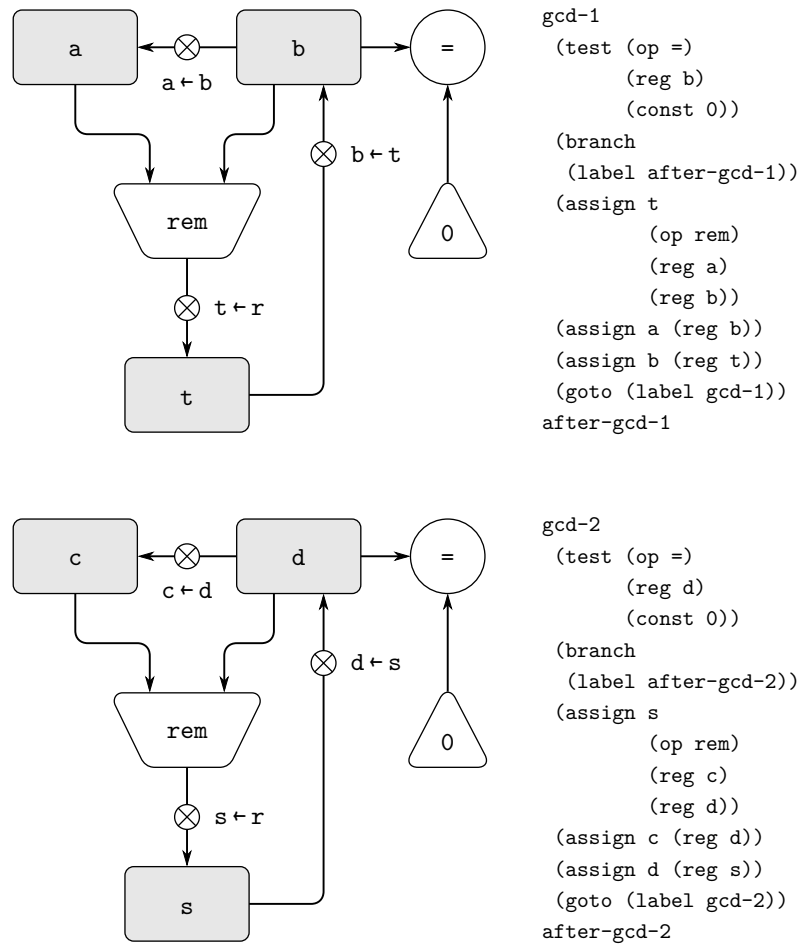
Figure 5.7 Portions of the data paths and controller sequence for a machine with two GCD computations.
