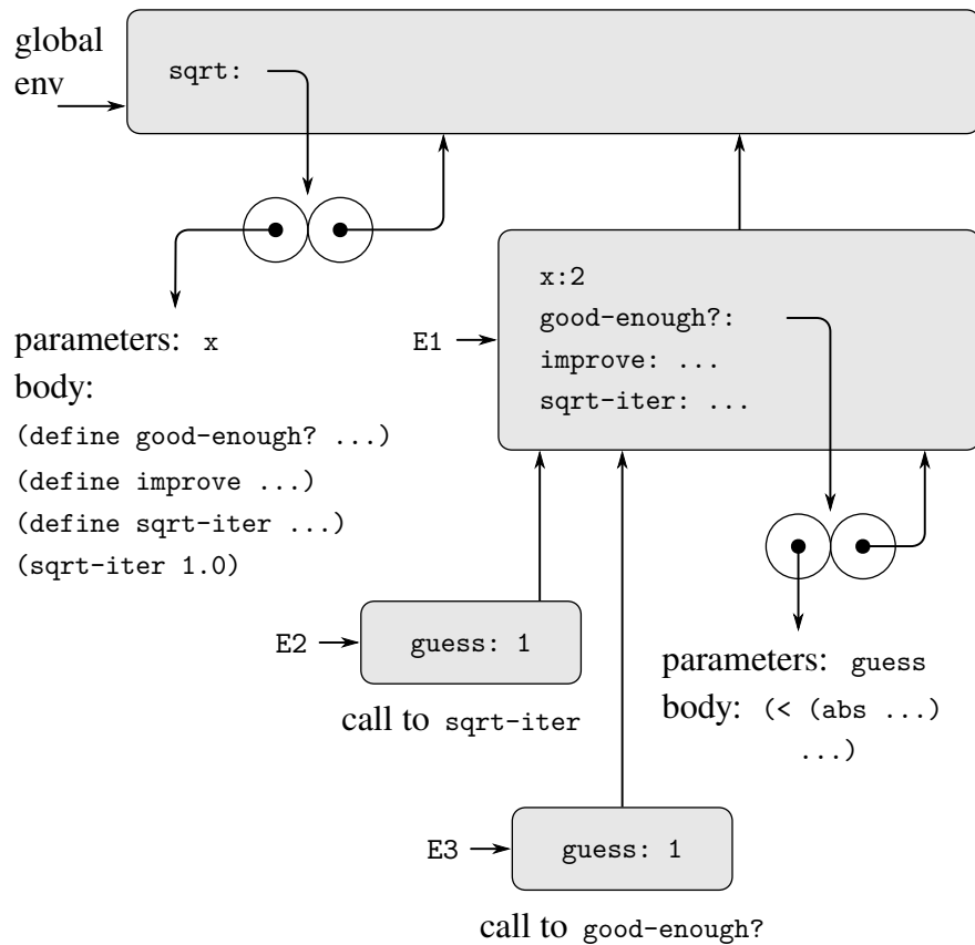
Figure 3.11 sqrt procedure with internal definitions.
