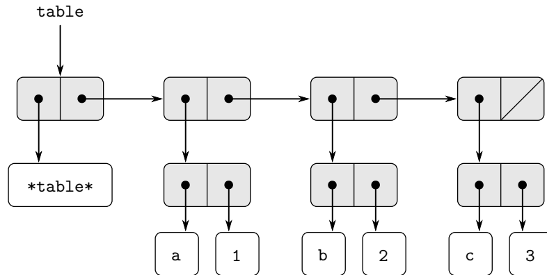
Figure 3.22 A table represented as a headed list.
