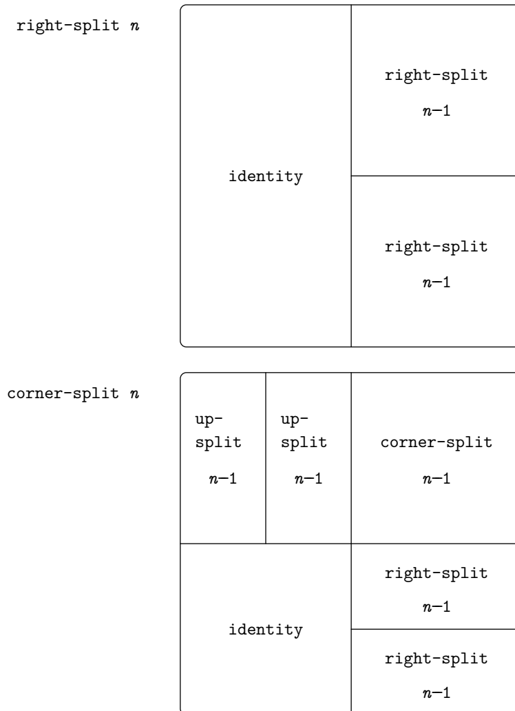
Figure 2.13 Recursive plans for right-split and corner-split.
