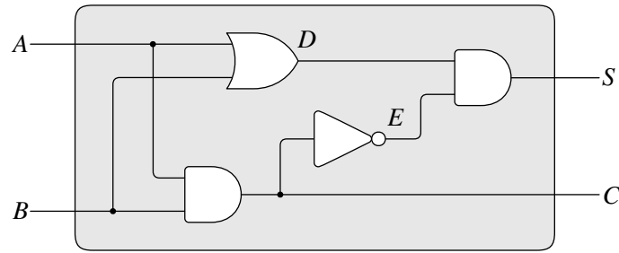
Figure 3.25 A half-adder circuit.
