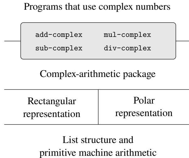
Figure 2.19 Data-abstraction barriers in the complex-number system.
