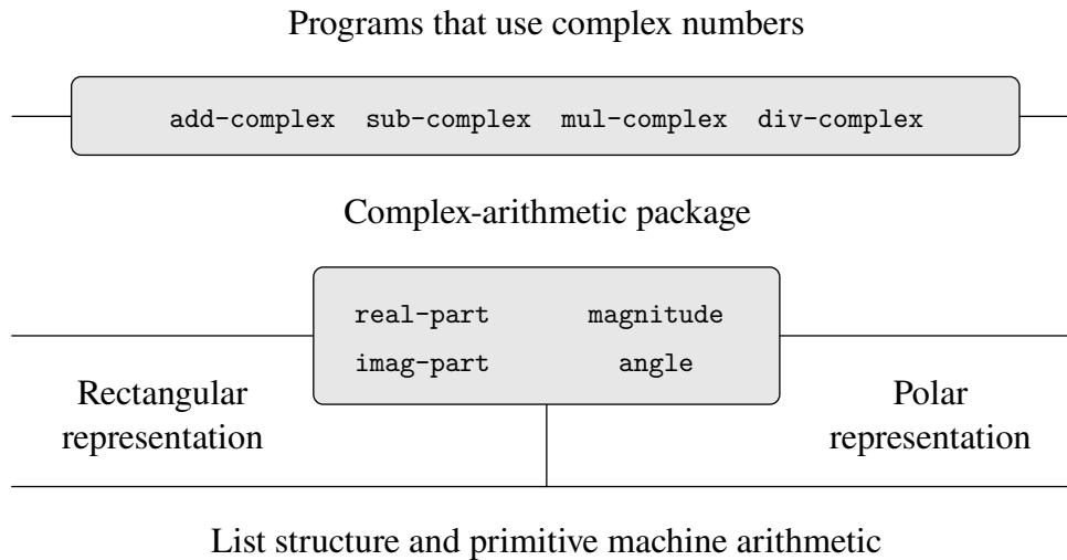
Figure 2.21 Structure of the generic complex-arithmetic system.
