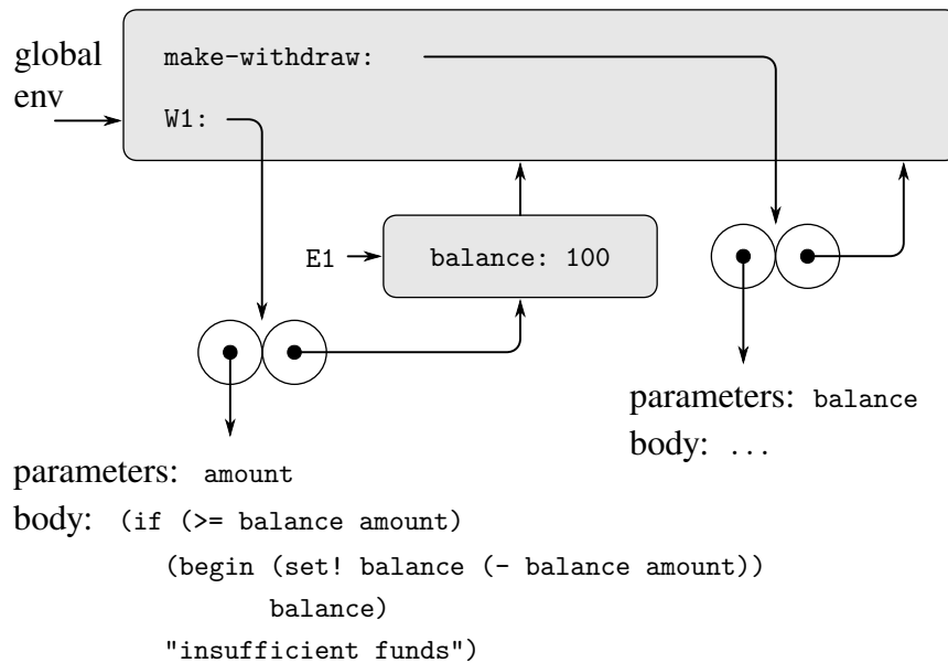
Figure 3.7 Result of evaluating (define W1 (make-withdraw 100)) .
