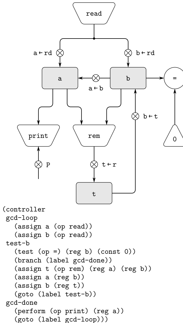
Figure 5.4 A GCD machine that reads inputs and prints results.
