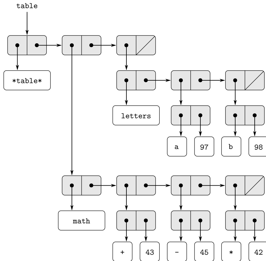
Figure 3.23 A two-dimensional table.
