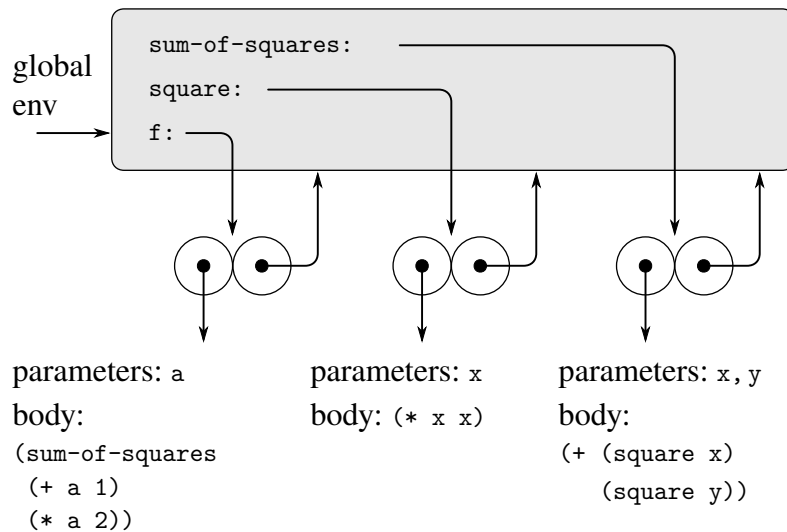
Figure 3.4 Procedure objects in the global frame.
