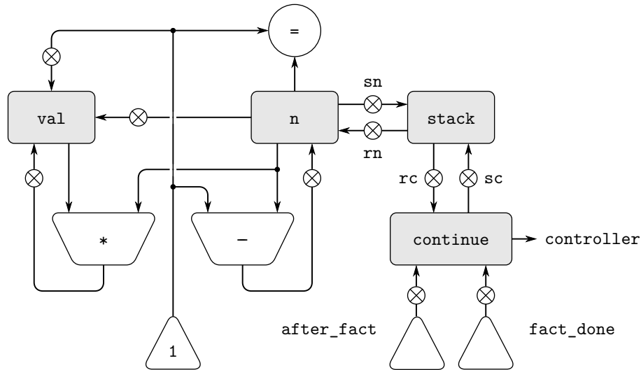
Figure 5.11 A recursive factorial machine.
