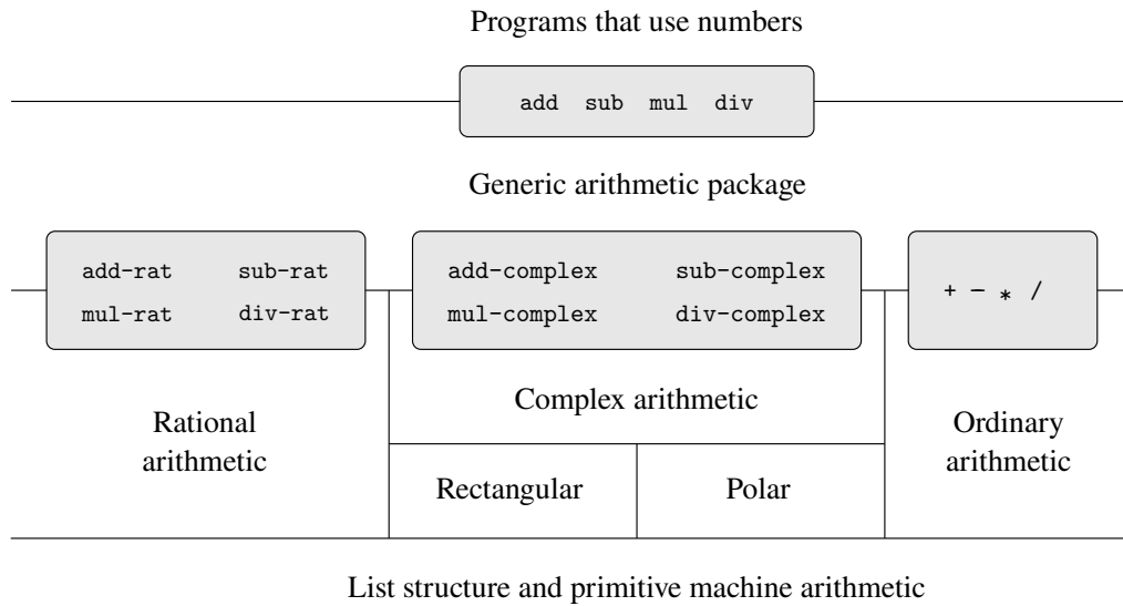
Figure 2.23 Generic arithmetic system.
