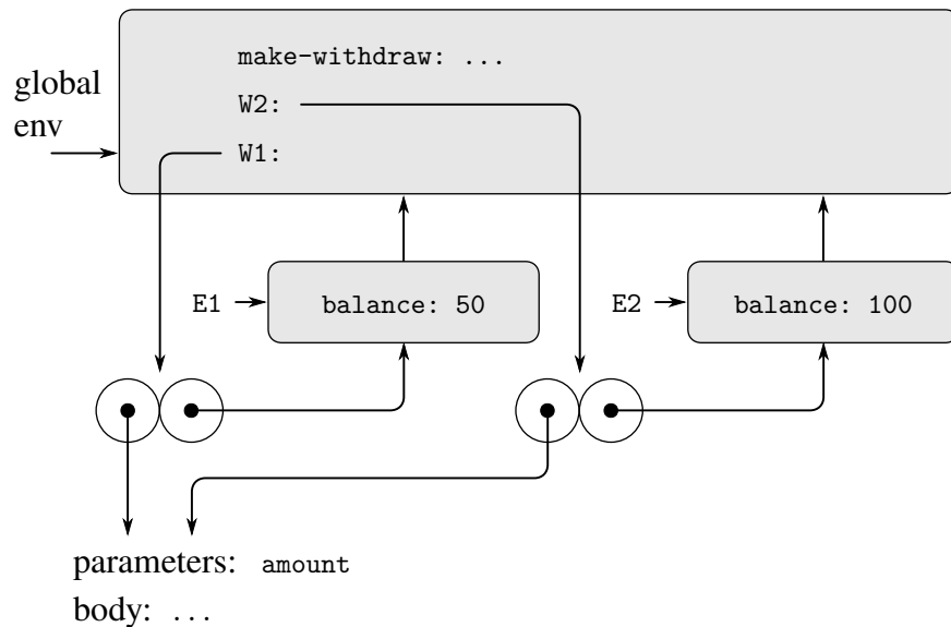
Figure 3.10 Using (define W2 (make-withdraw 100)) to create a second object.
