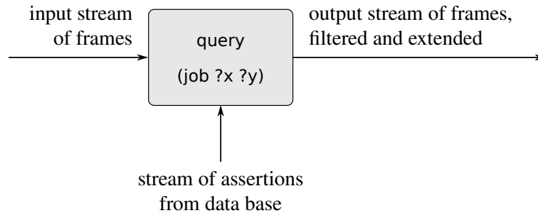
Figure 4.4 A query processes a stream of frames.
