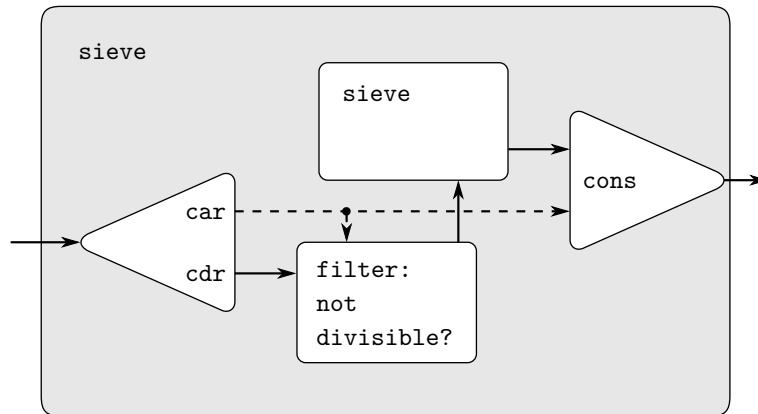
Figure 3.31 The prime sieve viewed as a signal-processing system. Each solid line represents a stream of values being transmitted. The dashed line from the car to the cons and the filter indicates that this is a single value rather than a stream.
