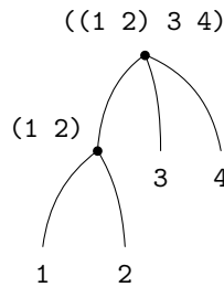
Figure 2.6 The list structure in figure 2.5 viewed as a tree.
