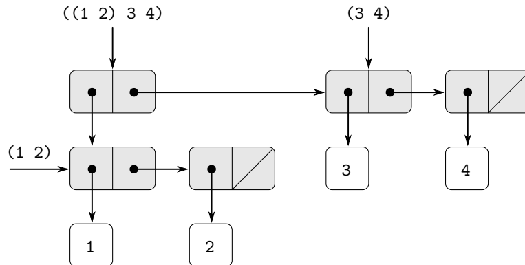
Figure 2.5 Structure formed by (cons (list 1 2) (list 3 4)).
