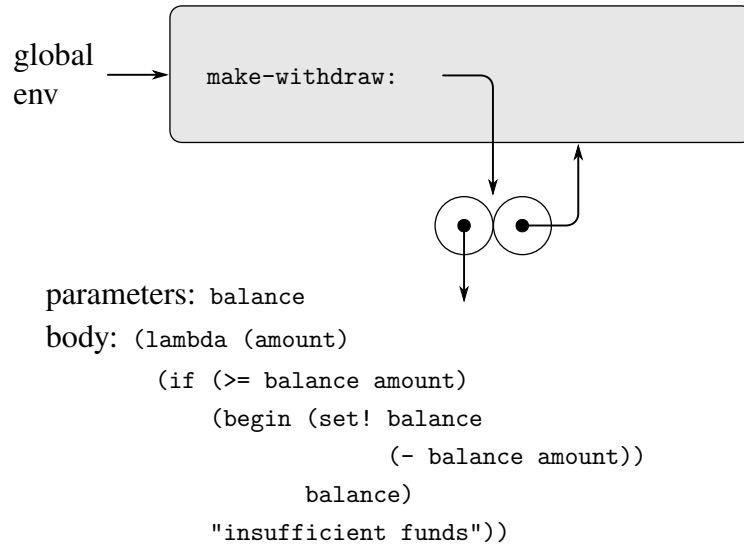
Figure 3.6 Result of defining make-withdraw in the global environment.
