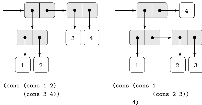
Figure 2.3 Two ways to combine 1, 2, 3, and 4 using pairs.
