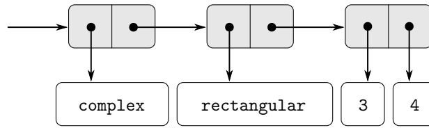
Figure 2.24 Representation of 3 + 4i in rectangular form.
