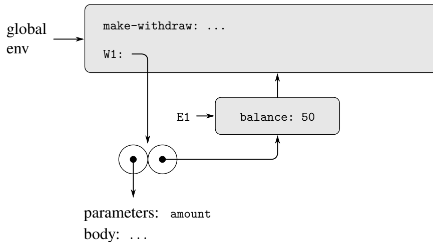
Figure 3.9 Environments after the call to W1.
