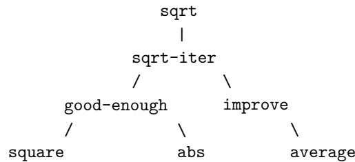
Figure 1.2 Procedural decomposition of the sqrt program.
