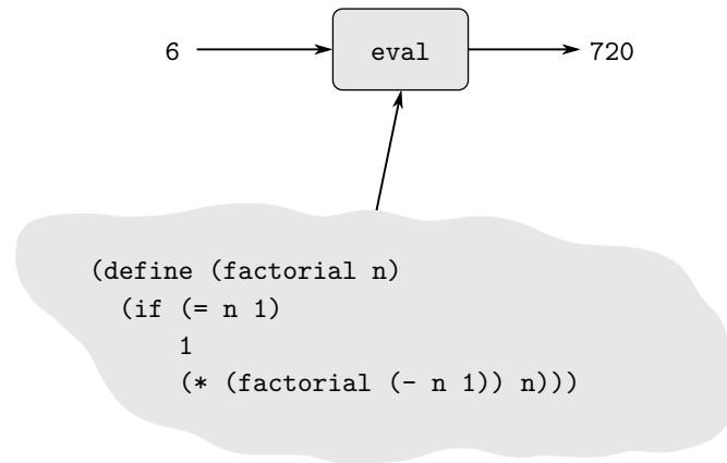
Figure 4.3 The evaluator emulating a factorial machine.
