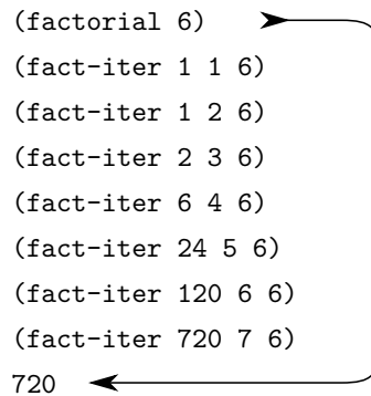
Figure 1.4 A linear iterative process for computing 6!.
