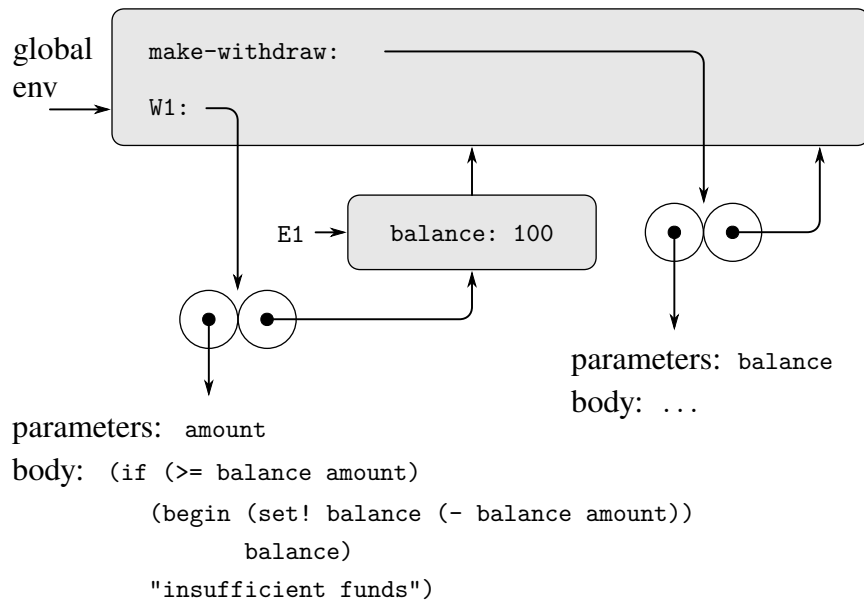
Figure 3.7 Result of evaluating (define W1 (make-withdraw 100)) .
