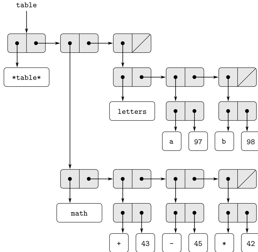
Figure 3.23 A two-dimensional table.
