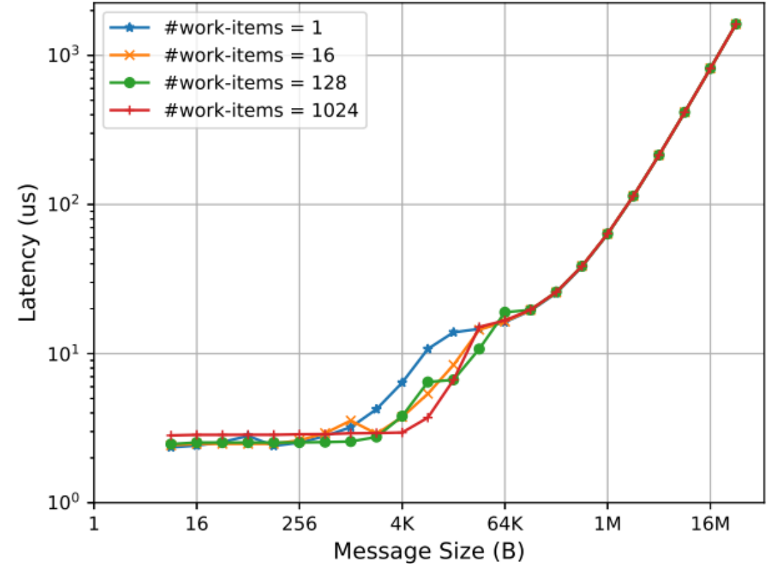
Put Work-Group Latency
