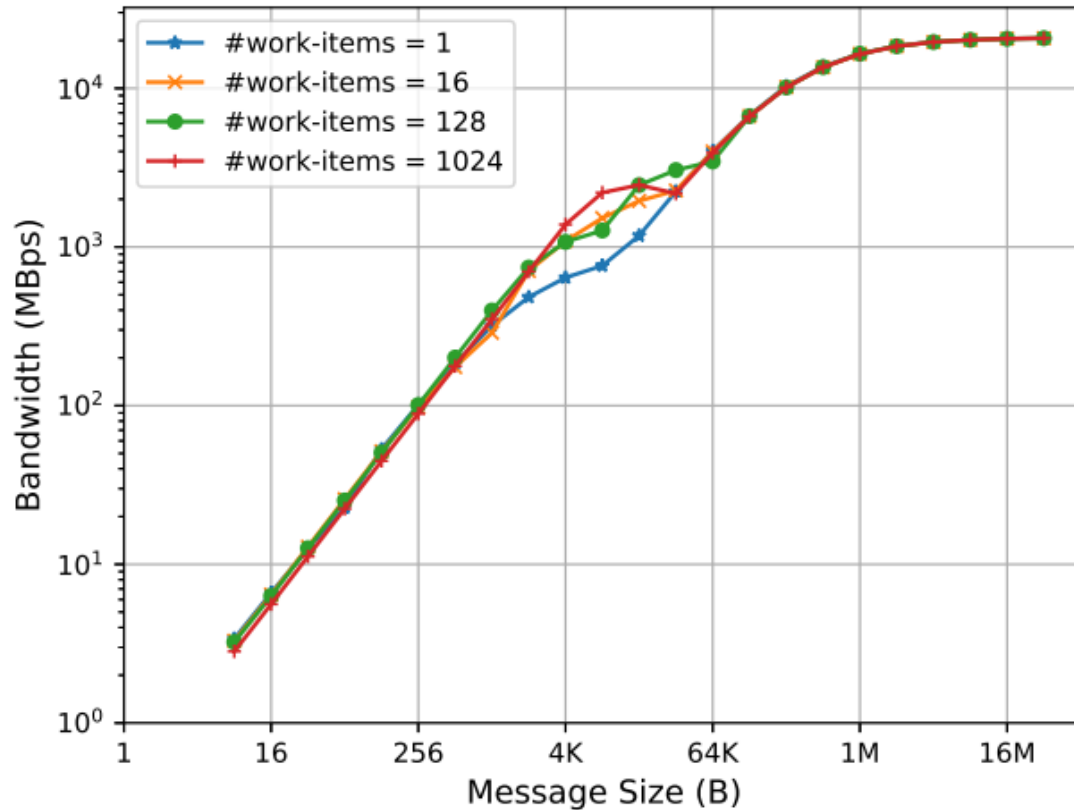
Put Work-Group Bandwidth
