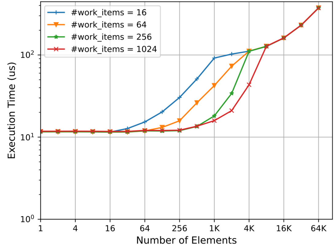
Fcollect WG (12 PEs) – w/ cutover tuning
