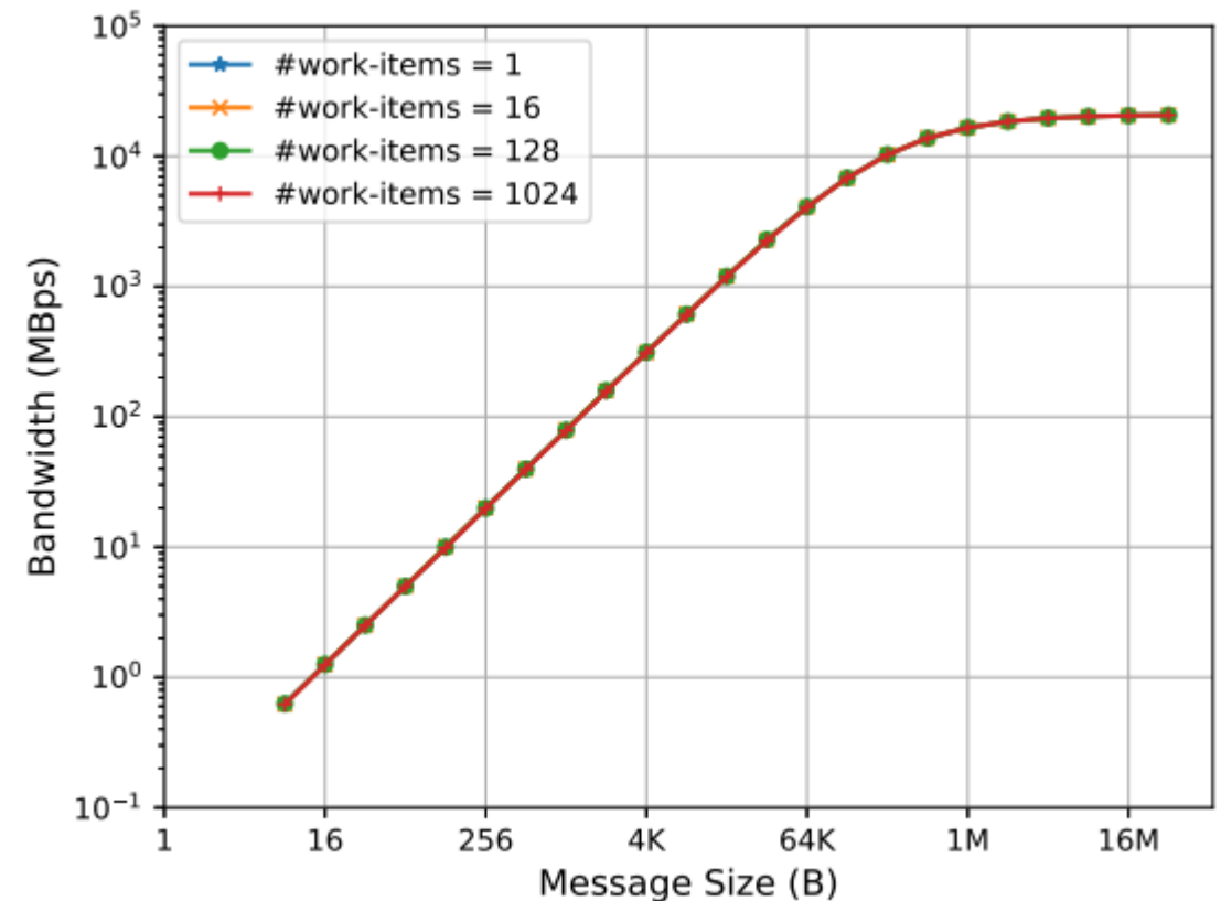
Copy engine transfer
