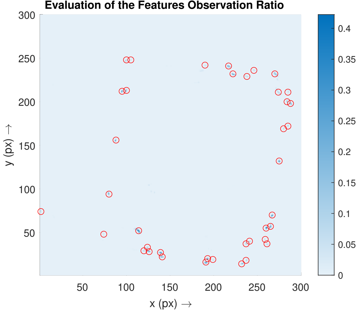
Figure 4.4: Evaluation of the features observation ratio, considering the robot pose along time, the Field-Of-View (FOV) of the 2D laser scanner, and a map resolution of 0.03 m/px.
