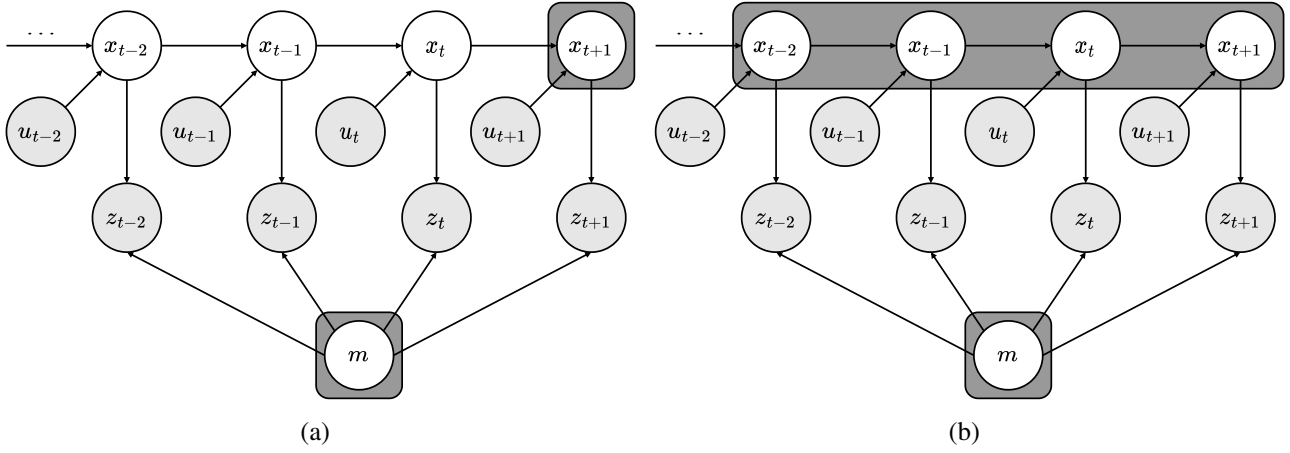
Figure 2.1: Graphical model of the Simultaneous Localization and Mapping (SLAM) problem: (a) online SLAM; (b) full SLAM [78]. Light gray circles represent observed inputs (measurements z_{1:t} and control variables u_{1:t} ), while nodes enclosed in a rounded rectangle indicate the jointly estimated variables: in (a), only the current pose x_t and the map m ; in (b), the entire trajectory x_{1:t} alongside the map m .
