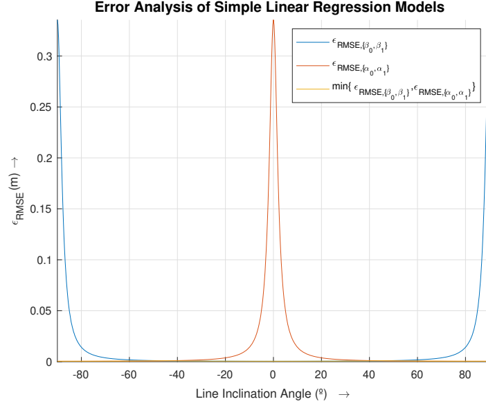
Figure 4.1: Error analysis of simple line regression models evaluating the fitting Root Mean Square Error (RMSE) , \epsilon_{RMSE} , for lines with an inclination angle between -90^\circ and 90^\circ and a simulation step of 0.25^\circ , a set of 100 data points equally distributed along each line, a distance Gaussian noise added to the data point coordinates of zero mean and 0.03 m standard deviation (same specifications as the Hokuyo UST-10LX sensor), and 1000 simulation samples per line [66].
